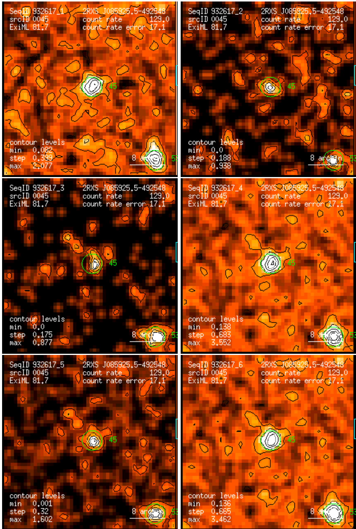
Figure 45: RASS 932617: detection 0045: band rate images, Gaussian filter: (1) PSPC channels 11 – 41, (2) 52 – 90, (3) 91 – 201, (4) 11 – 235, (5) 52 – 201, (6) 11 – 201. Broad band rates in counts/ks. Band rate contour levels in counts/ks/arcmin 2 .
