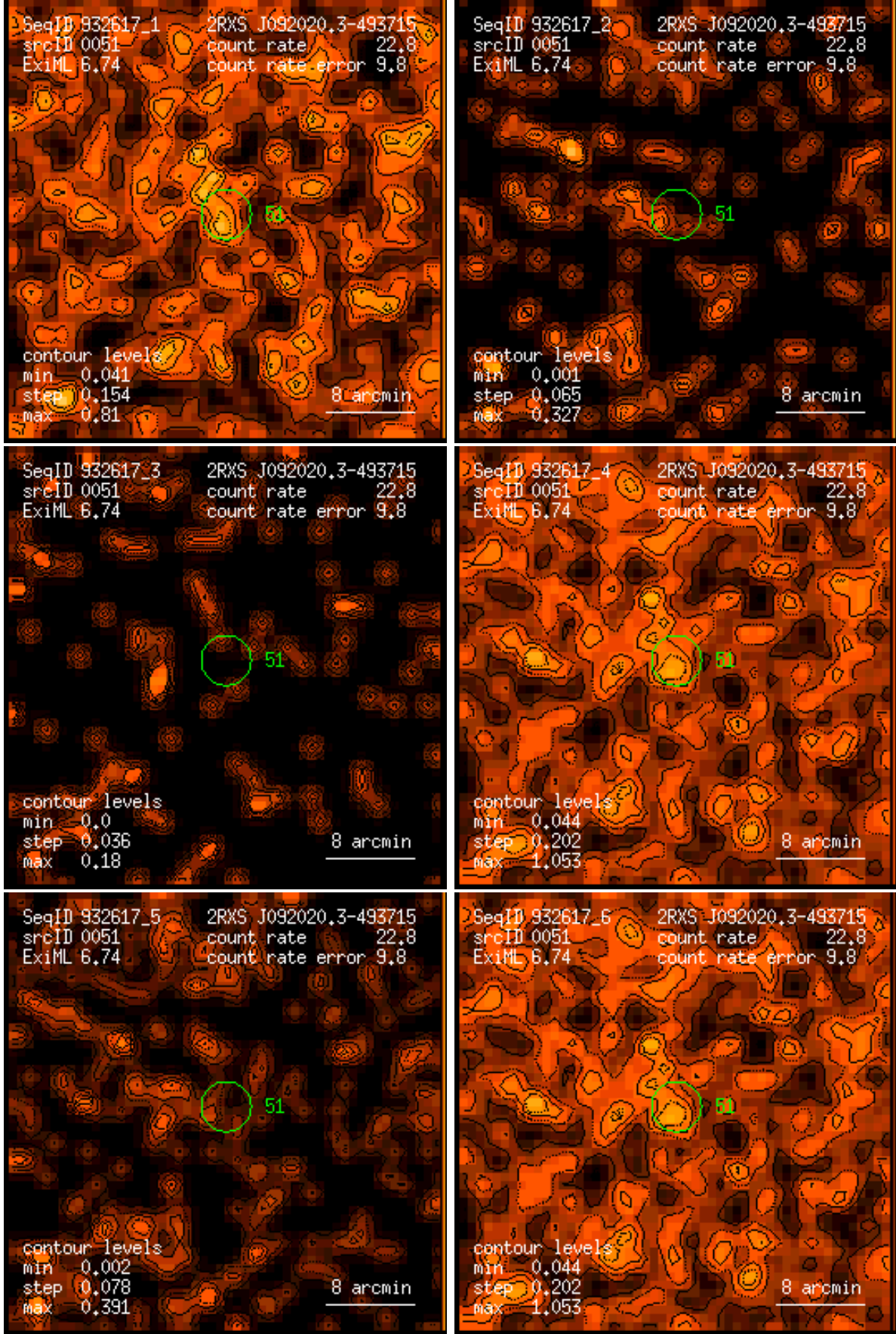
Figure 51: RASS 932617: detection 0051: band rate images, Gaussian filter: (1) PSPC channels 11 – 41, (2) 52 – 90, (3) 91 – 201, (4) 11 – 235, (5) 52 – 201, (6) 11 – 201. Broad band rates in counts/ks. Band rate contour levels in counts/ks/arcmin 2 .
