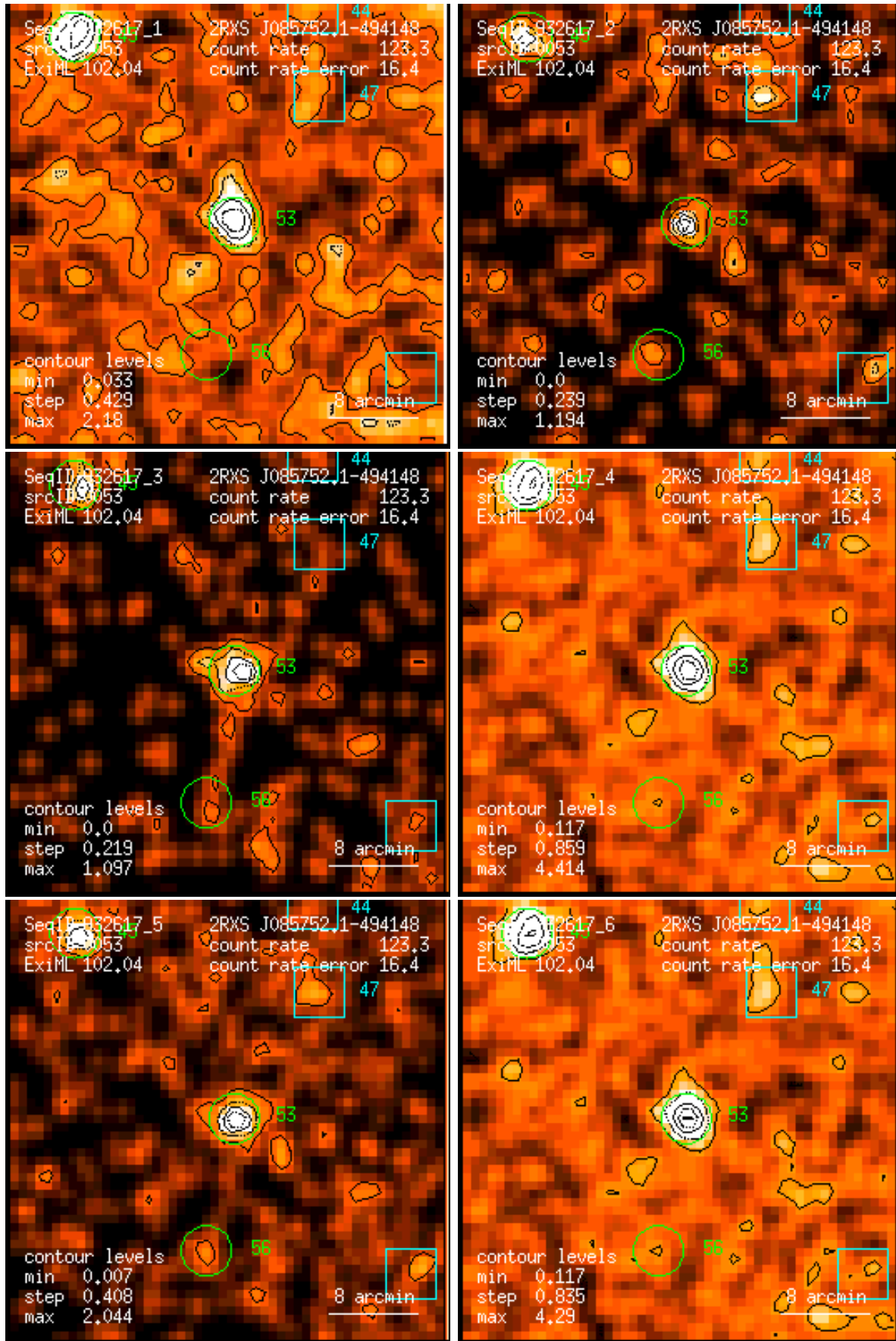
Figure 53: RASS 932617: detection 0053: band rate images, Gaussian filter: (1) PSPC channels 11 – 41, (2) 52 – 90, (3) 91 – 201, (4) 11 – 235, (5) 52 – 201, (6) 11 – 201. Broad band rates in counts/ks. Band rate contour levels in counts/ks/arcmin 2 .
