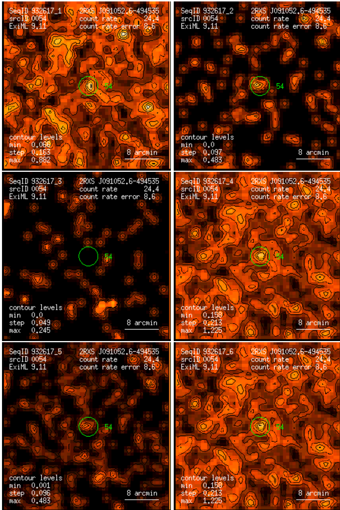
Figure 54: RASS 932617: detection 0054: band rate images, Gaussian filter: (1) PSPC channels 11 – 41, (2) 52 – 90, (3) 91 – 201, (4) 11 – 235, (5) 52 – 201, (6) 11 – 201. Broad band rates in counts/ks. Band rate contour levels in counts/ks/arcmin 2 .
