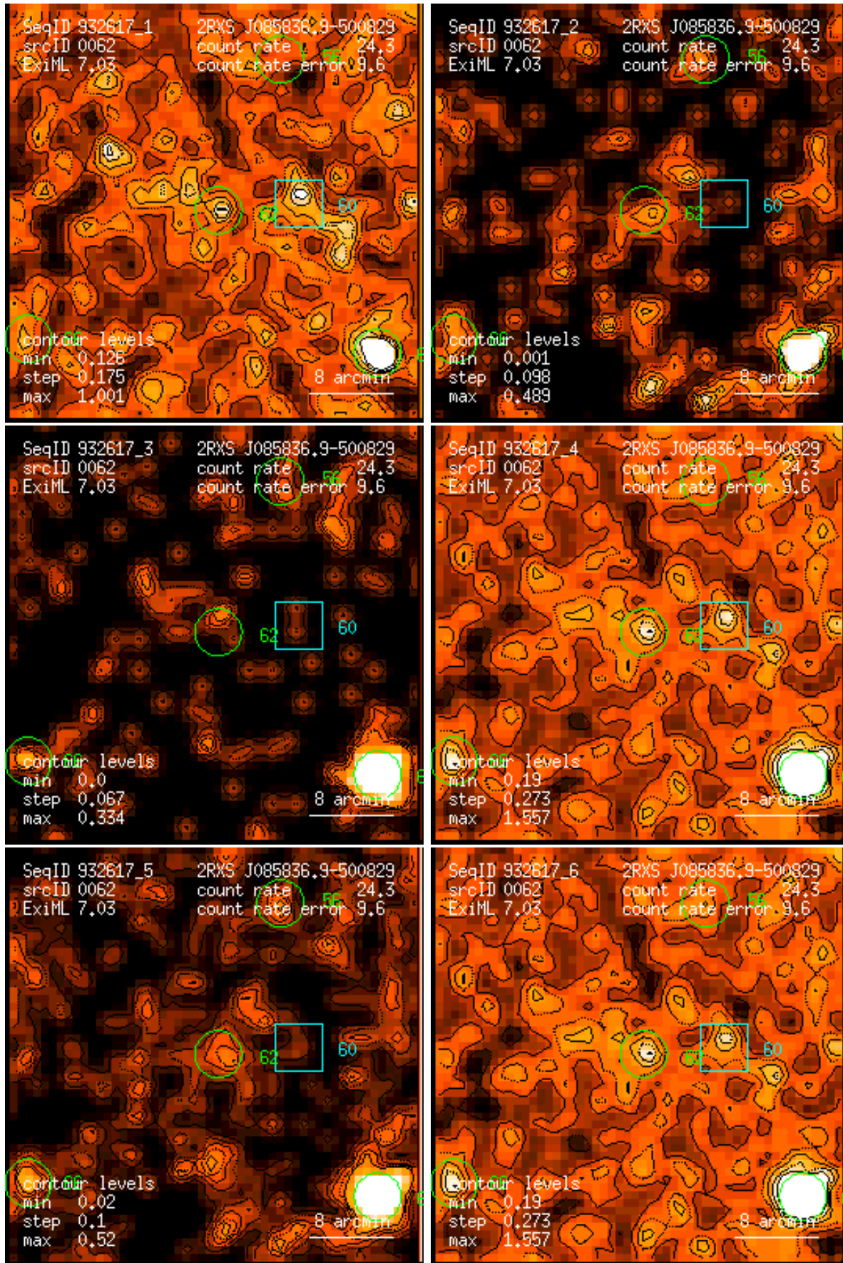
Figure 62: RASS 932617: detection 0062: band rate images, Gaussian filter: (1) PSPC channels 11 – 41, (2) 52 – 90, (3) 91 – 201, (4) 11 – 235, (5) 52 – 201, (6) 11 – 201. Broad band rates in counts/ks. Band rate contour levels in counts/ks/arcmin 2 .
