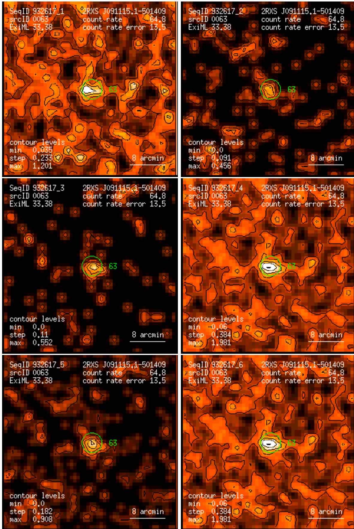
Figure 63: RASS 932617: detection 0063: band rate images, Gaussian filter: (1) PSPC channels 11 – 41, (2) 52 – 90, (3) 91 – 201, (4) 11 – 235, (5) 52 – 201, (6) 11 – 201. Broad band rates in counts/ks. Band rate contour levels in counts/ks/arcmin 2 .
