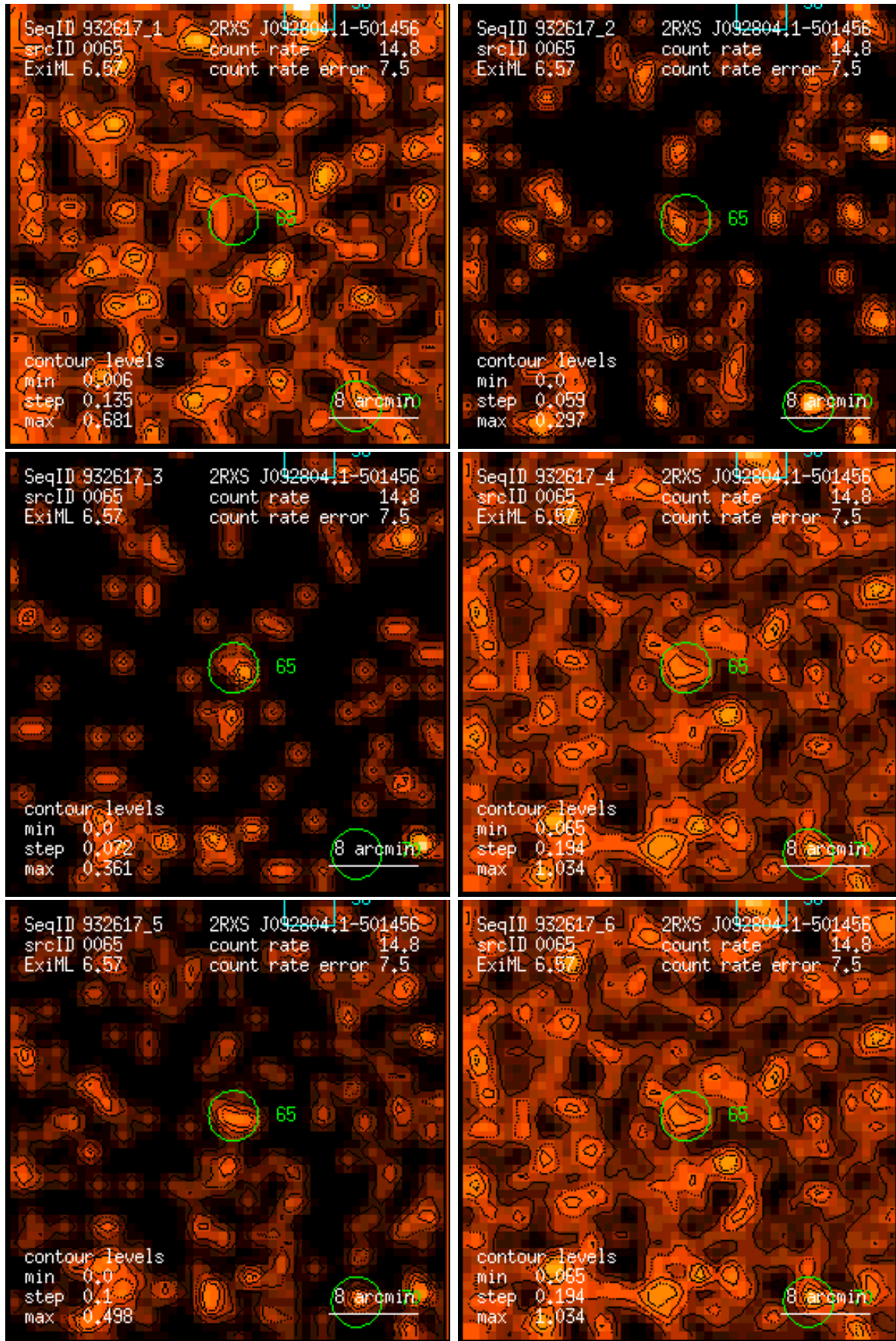
Figure 65: RASS 932617: detection 0065: band rate images, Gaussian filter: (1) PSPC channels 11 – 41, (2) 52 – 90, (3) 91 – 201, (4) 11 – 235, (5) 52 – 201, (6) 11 – 201. Broad band rates in counts/ks. Band rate contour levels in counts/ks/arcmin 2 .
