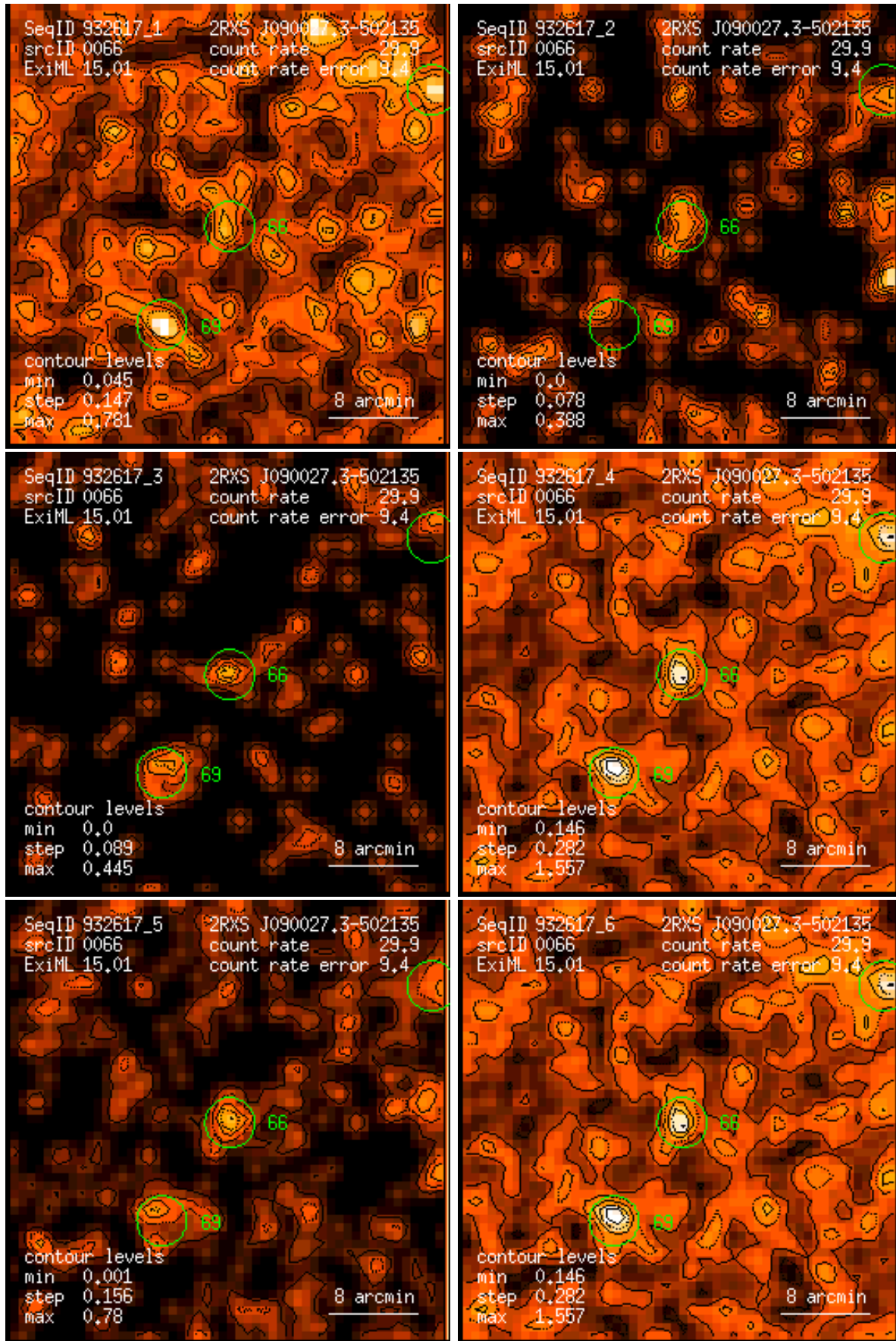
Figure 66: RASS 932617: detection 0066: band rate images, Gaussian filter: (1) PSPC channels 11 – 41, (2) 52 – 90, (3) 91 – 201, (4) 11 – 235, (5) 52 – 201, (6) 11 – 201. Broad band rates in counts/ks. Band rate contour levels in counts/ks/arcmin 2 .
