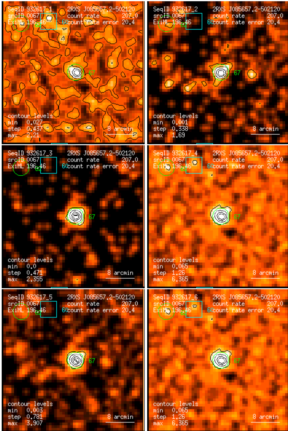
Figure 67: RASS 932617: detection 0067: band rate images, Gaussian filter: (1) PSPC channels 11 – 41, (2) 52 – 90, (3) 91 – 201, (4) 11 – 235, (5) 52 – 201, (6) 11 – 201. Broad band rates in counts/ks. Band rate contour levels in counts/ks/arcmin 2 .
