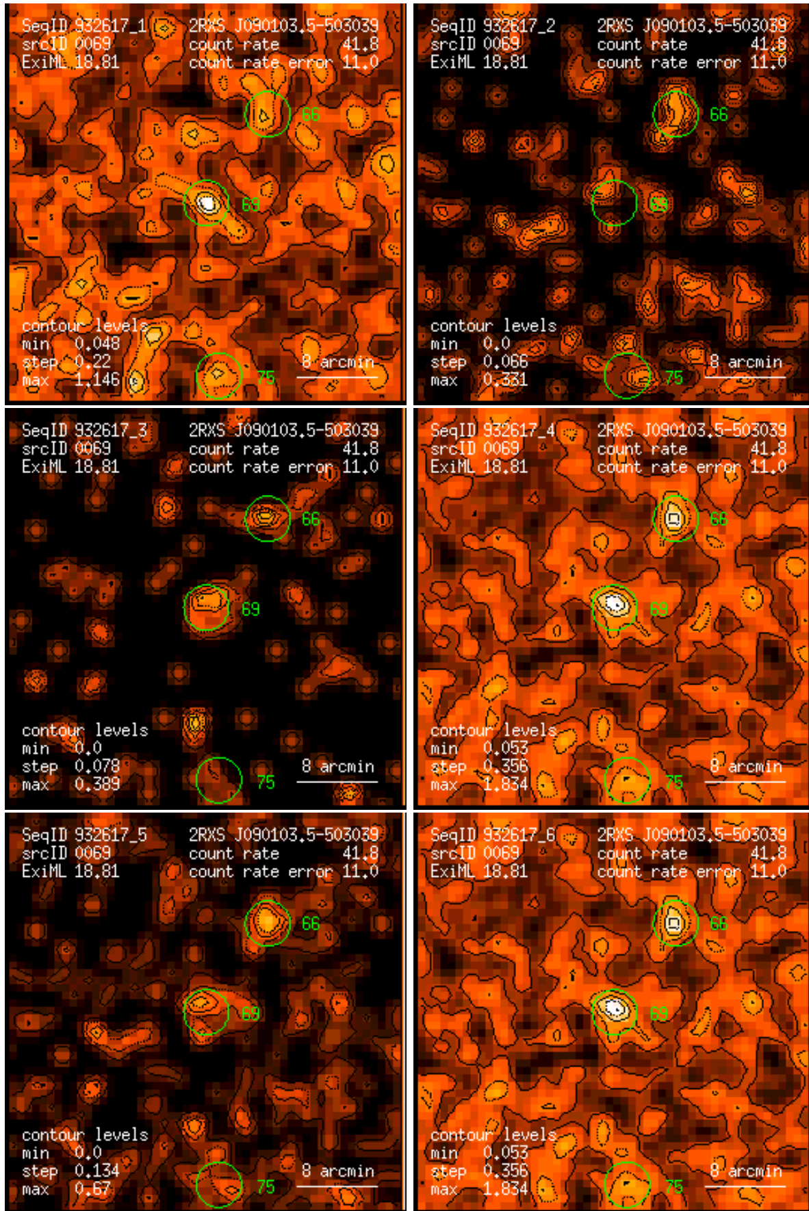
Figure 69: RASS 932617: detection 0069: band rate images, Gaussian filter: (1) PSPC channels 11 – 41, (2) 52 – 90, (3) 91 – 201, (4) 11 – 235, (5) 52 – 201, (6) 11 – 201. Broad band rates in counts/ks. Band rate contour levels in counts/ks/arcmin 2 .
