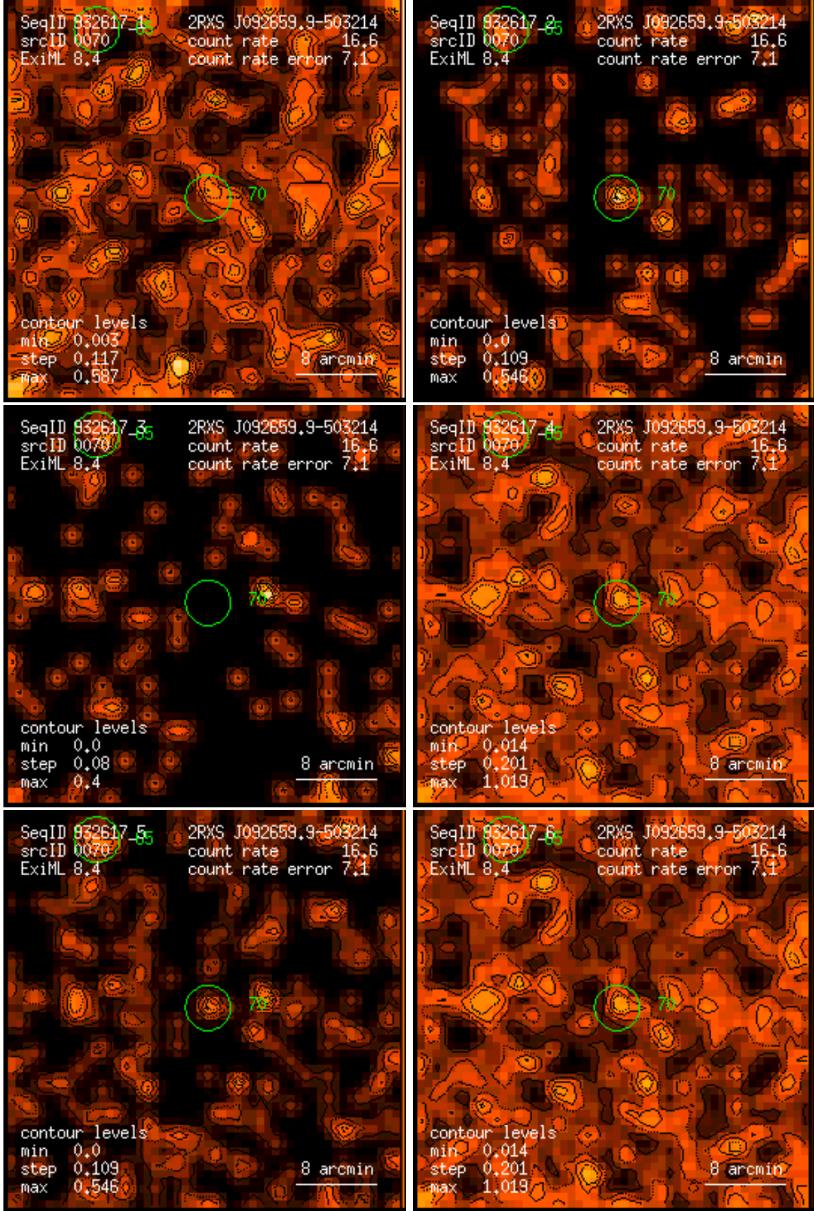
Figure 70: RASS 932617: detection 0070: band rate images, Gaussian filter: (1) PSPC channels 11 – 41, (2) 52 – 90, (3) 91 – 201, (4) 11 – 235, (5) 52 – 201, (6) 11 – 201. Broad band rates in counts/ks. Band rate contour levels in counts/ks/arcmin 2 .
