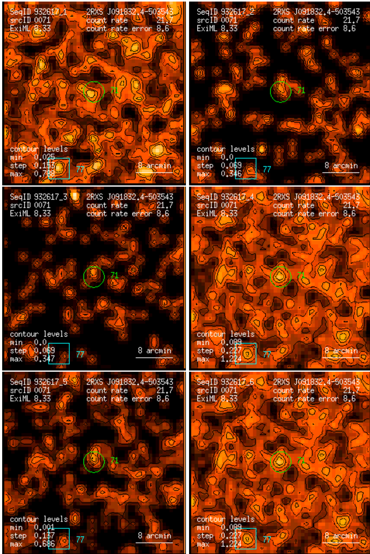
Figure 71: RASS 932617: detection 0071: band rate images, Gaussian filter: (1) PSPC channels 11 – 41, (2) 52 – 90, (3) 91 – 201, (4) 11 – 235, (5) 52 – 201, (6) 11 – 201. Broad band rates in counts/ks. Band rate contour levels in counts/ks/arcmin 2 .
