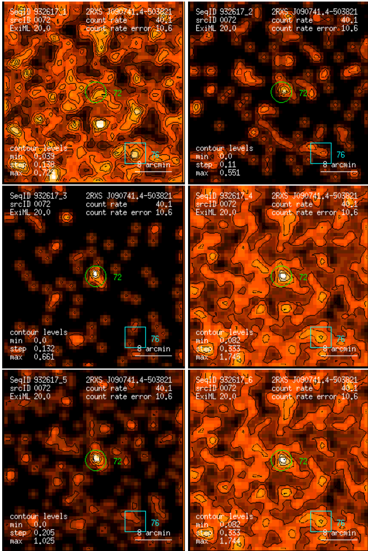
Figure 72: RASS 932617: detection 0072: band rate images, Gaussian filter: (1) PSPC channels 11 – 41, (2) 52 – 90, (3) 91 – 201, (4) 11 – 235, (5) 52 – 201, (6) 11 – 201. Broad band rates in counts/ks. Band rate contour levels in counts/ks/arcmin 2 .
