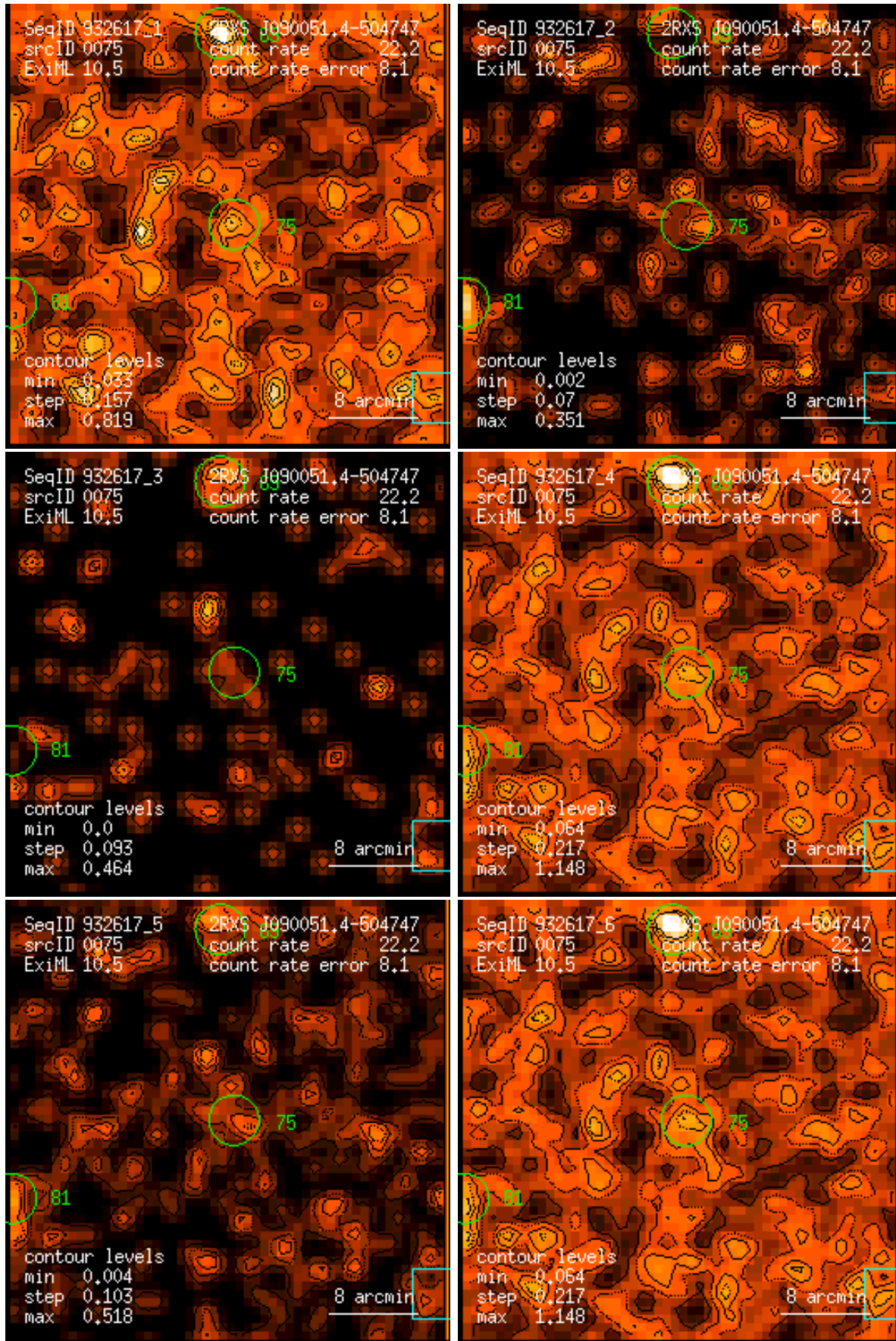
Figure 75: RASS 932617: detection 0075: band rate images, Gaussian filter: (1) PSPC channels 11 – 41, (2) 52 – 90, (3) 91 – 201, (4) 11 – 235, (5) 52 – 201, (6) 11 – 201. Broad band rates in counts/ks. Band rate contour levels in counts/ks/arcmin 2 .
