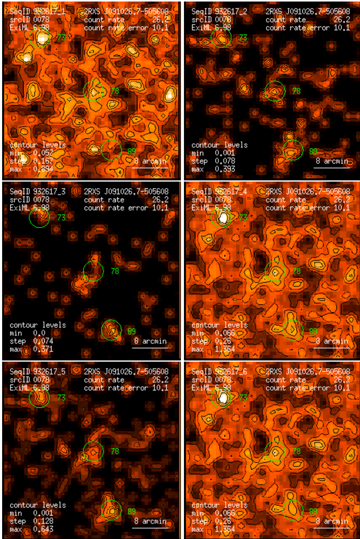
Figure 78: RASS 932617: detection 0078: band rate images, Gaussian filter: (1) PSPC channels 11 – 41, (2) 52 – 90, (3) 91 – 201, (4) 11 – 235, (5) 52 – 201, (6) 11 – 201. Broad band rates in counts/ks. Band rate contour levels in counts/ks/arcmin 2 .
