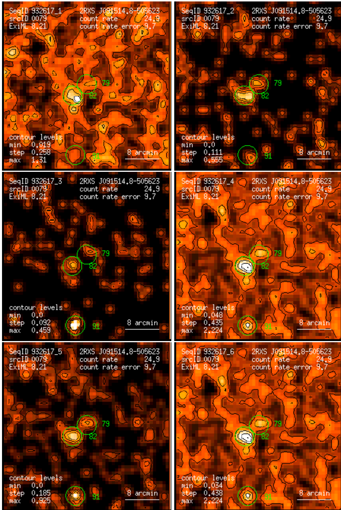
Figure 79: RASS 932617: detection 0079: band rate images, Gaussian filter: (1) PSPC channels 11 – 41, (2) 52 – 90, (3) 91 – 201, (4) 11 – 235, (5) 52 – 201, (6) 11 – 201. Broad band rates in counts/ks. Band rate contour levels in counts/ks/arcmin 2 .
