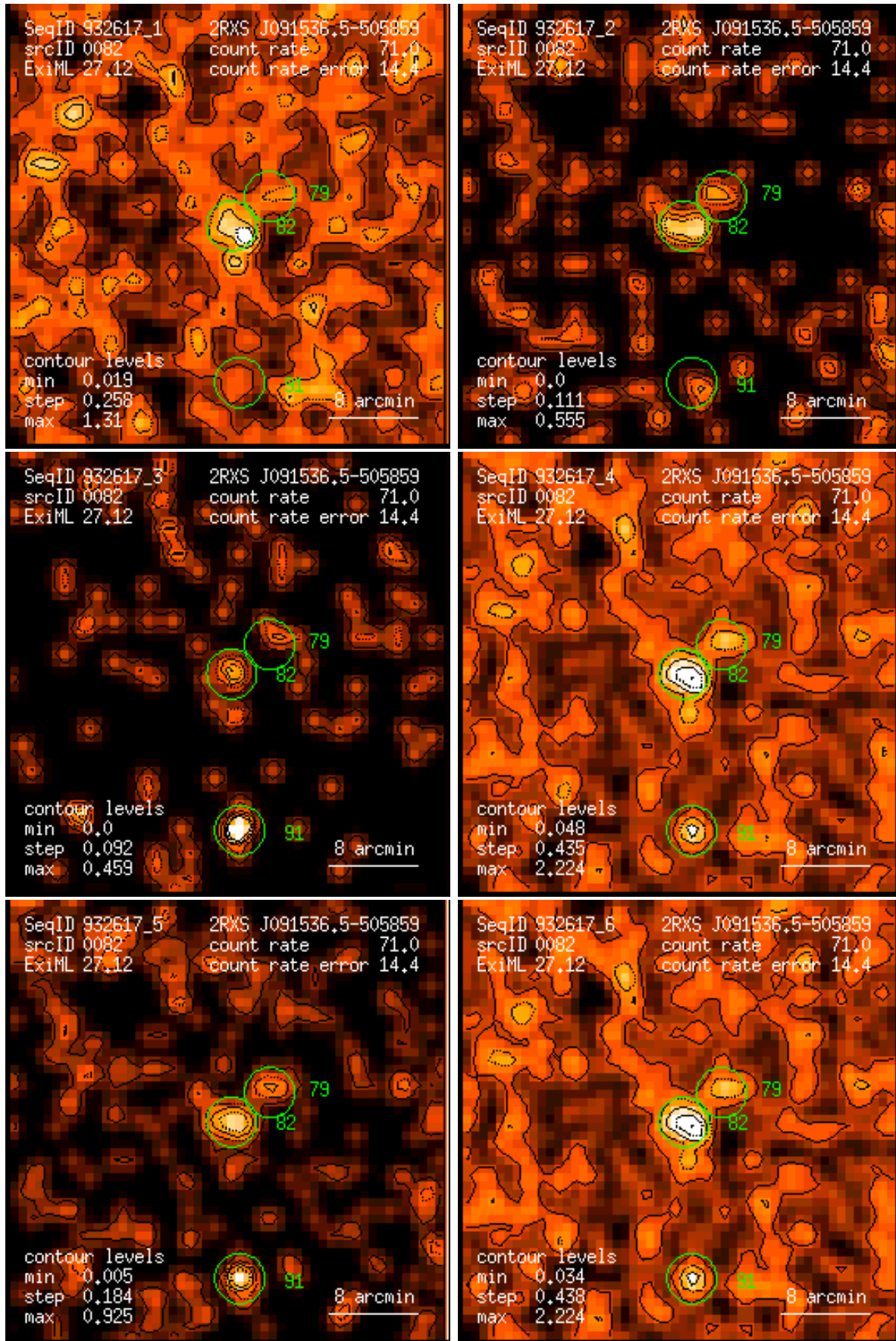
Figure 82: RASS 932617: detection 0082: band rate images, Gaussian filter: (1) PSPC channels 11 – 41, (2) 52 – 90, (3) 91 – 201, (4) 11 – 235, (5) 52 – 201, (6) 11 – 201. Broad band rates in counts/ks. Band rate contour levels in counts/ks/arcmin 2 .
