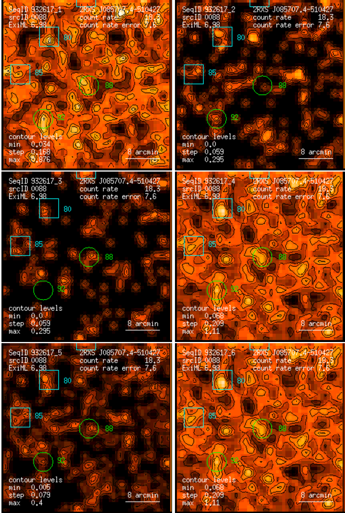
Figure 88: RASS 932617: detection 0088: band rate images, Gaussian filter: (1) PSPC channels 11 – 41, (2) 52 – 90, (3) 91 – 201, (4) 11 – 235, (5) 52 – 201, (6) 11 – 201. Broad band rates in counts/ks. Band rate contour levels in counts/ks/arcmin 2 .
