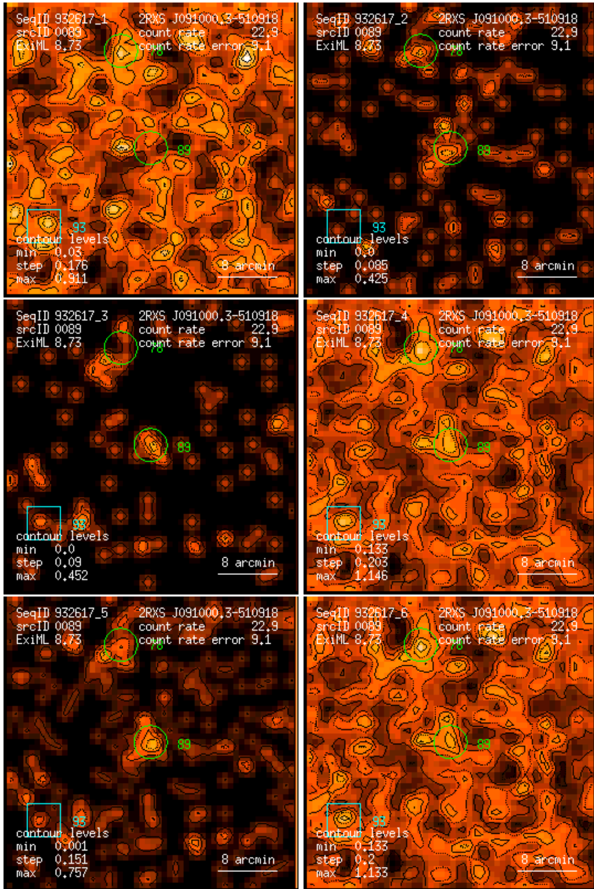
Figure 89: RASS 932617: detection 0089: band rate images, Gaussian filter: (1) PSPC channels 11 – 41, (2) 52 – 90, (3) 91 – 201, (4) 11 – 235, (5) 52 – 201, (6) 11 – 201. Broad band rates in counts/ks. Band rate contour levels in counts/ks/arcmin 2 .
