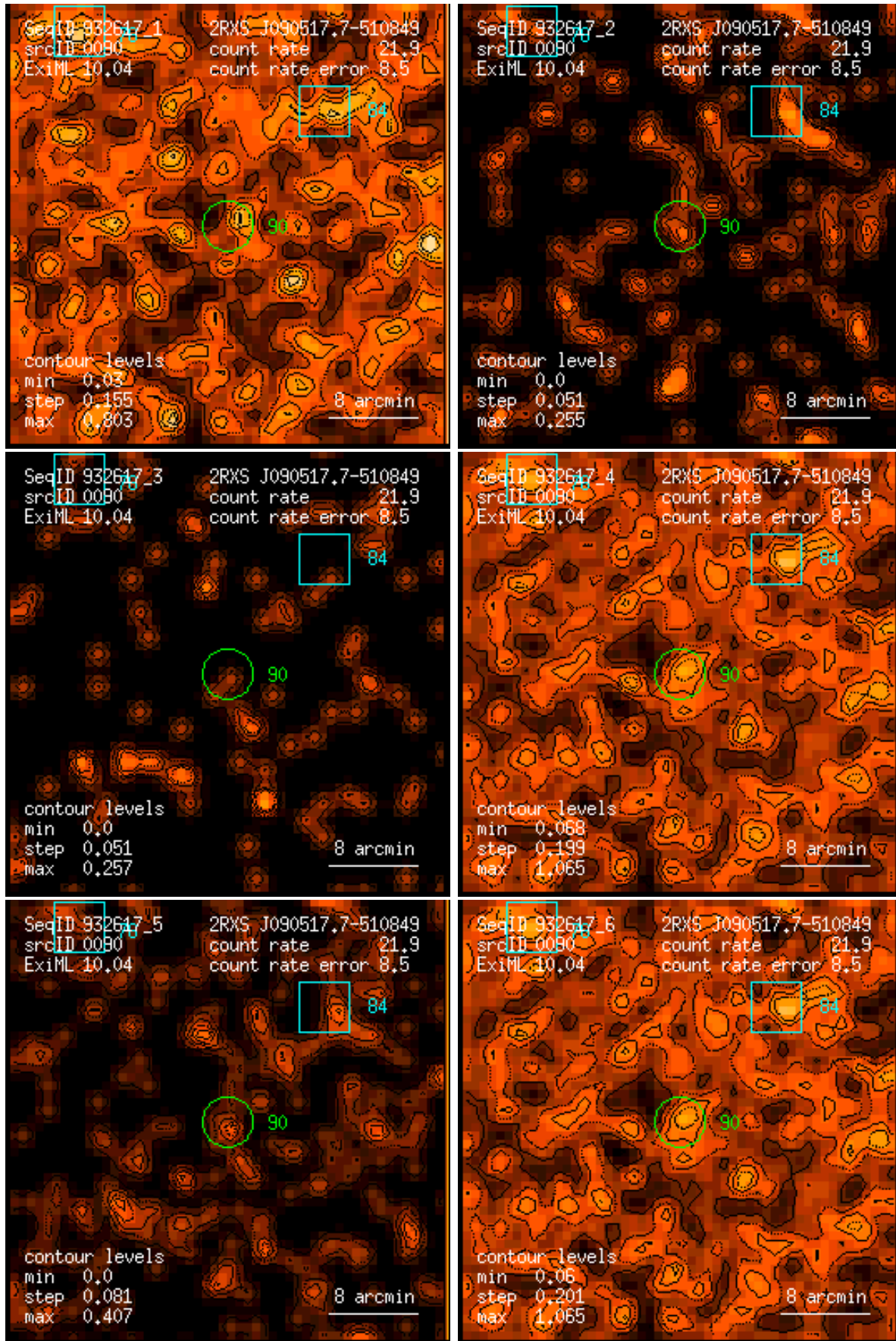
Figure 90: RASS 932617: detection 0090: band rate images, Gaussian filter: (1) PSPC channels 11 – 41, (2) 52 – 90, (3) 91 – 201, (4) 11 – 235, (5) 52 – 201, (6) 11 – 201. Broad band rates in counts/ks. Band rate contour levels in counts/ks/arcmin 2 .
