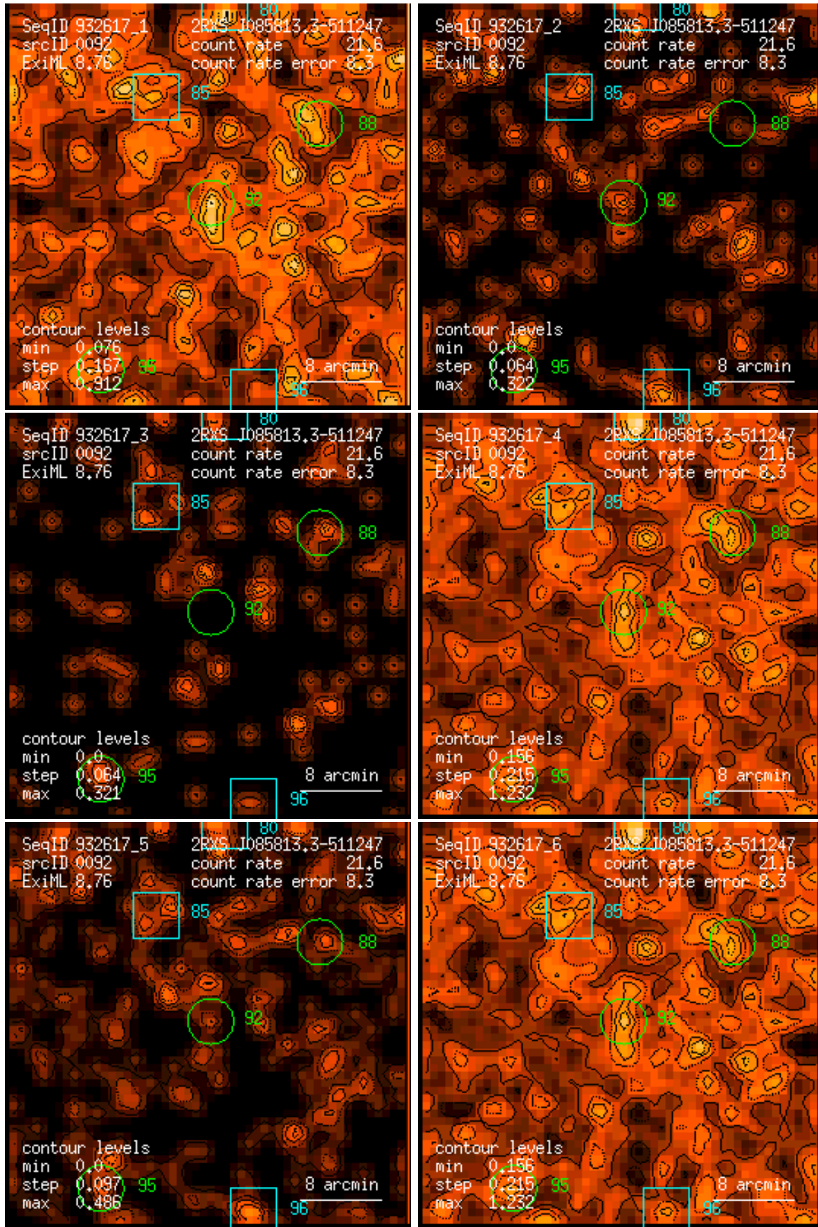
Figure 92: RASS 932617: detection 0092: band rate images, Gaussian filter: (1) PSPC channels 11 – 41, (2) 52 – 90, (3) 91 – 201, (4) 11 – 235, (5) 52 – 201, (6) 11 – 201. Broad band rates in counts/ks. Band rate contour levels in counts/ks/arcmin 2 .
