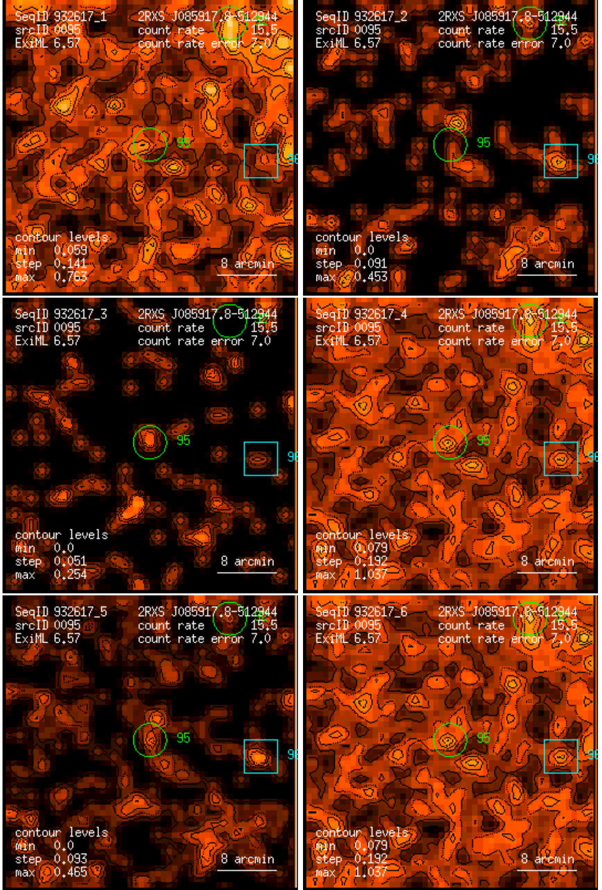
Figure 95: RASS 932617: detection 0095: band rate images, Gaussian filter: (1) PSPC channels 11 – 41, (2) 52 – 90, (3) 91 – 201, (4) 11 – 235, (5) 52 – 201, (6) 11 – 201. Broad band rates in counts/ks. Band rate contour levels in counts/ks/arcmin 2 .
