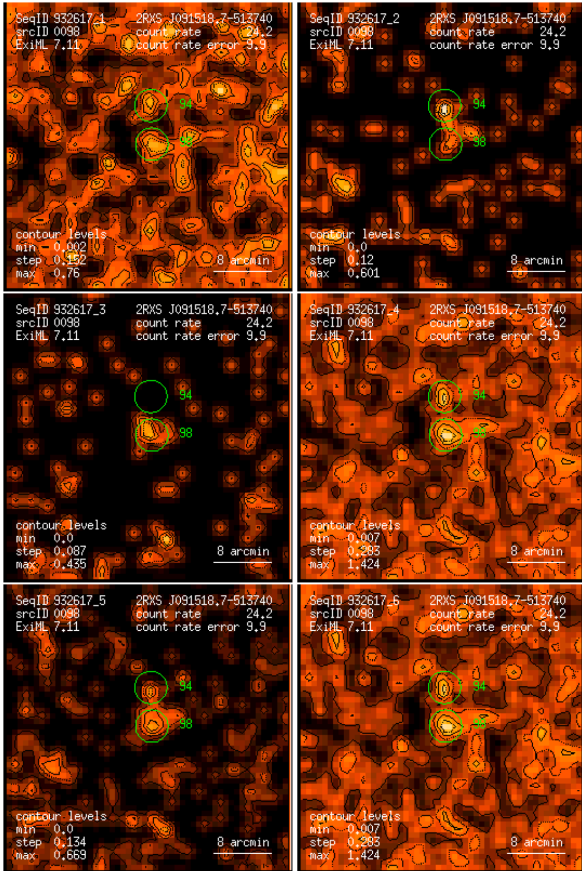
Figure 98: RASS 932617: detection 0098: band rate images, Gaussian filter: (1) PSPC channels 11 – 41, (2) 52 – 90, (3) 91 – 201, (4) 11 – 235, (5) 52 – 201, (6) 11 – 201. Broad band rates in counts/ks. Band rate contour levels in counts/ks/arcmin 2 .
