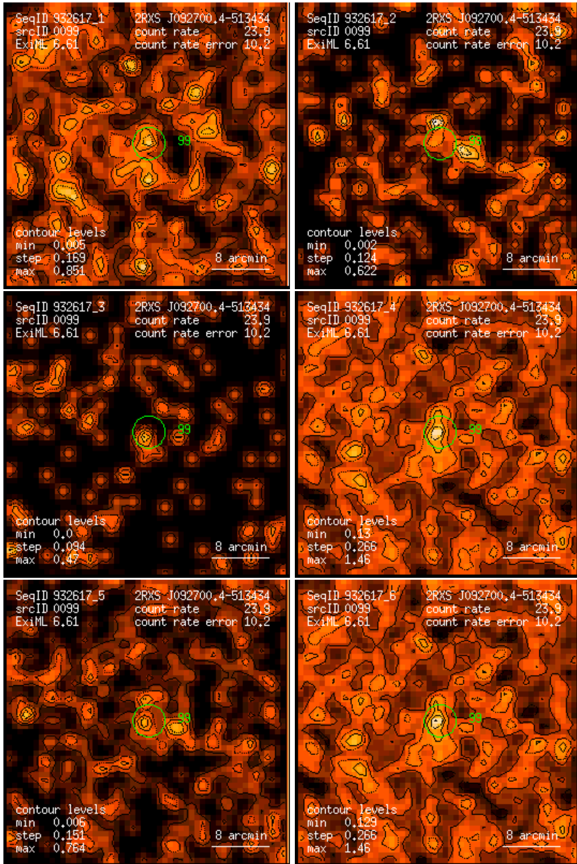
Figure 99: RASS 932617: detection 0099: band rate images, Gaussian filter: (1) PSPC channels 11 – 41, (2) 52 – 90, (3) 91 – 201, (4) 11 – 235, (5) 52 – 201, (6) 11 – 201. Broad band rates in counts/ks. Band rate contour levels in counts/ks/arcmin 2 .
