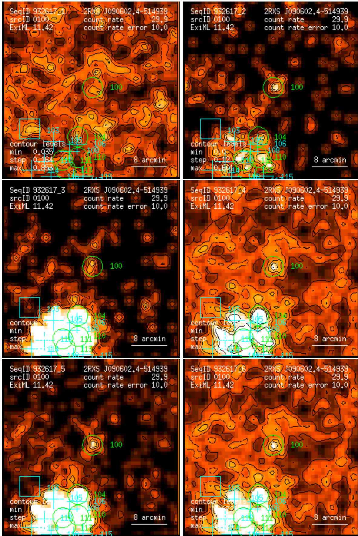
Figure 100: RASS 932617: detection 0100: band rate images, Gaussian filter: (1) PSPC channels 11 – 41, (2) 52 – 90, (3) 91 – 201, (4) 11 – 235, (5) 52 – 201, (6) 11 – 201. Broad band rates in counts/ks. Band rate contour levels in counts/ks/arcmin 2 .
