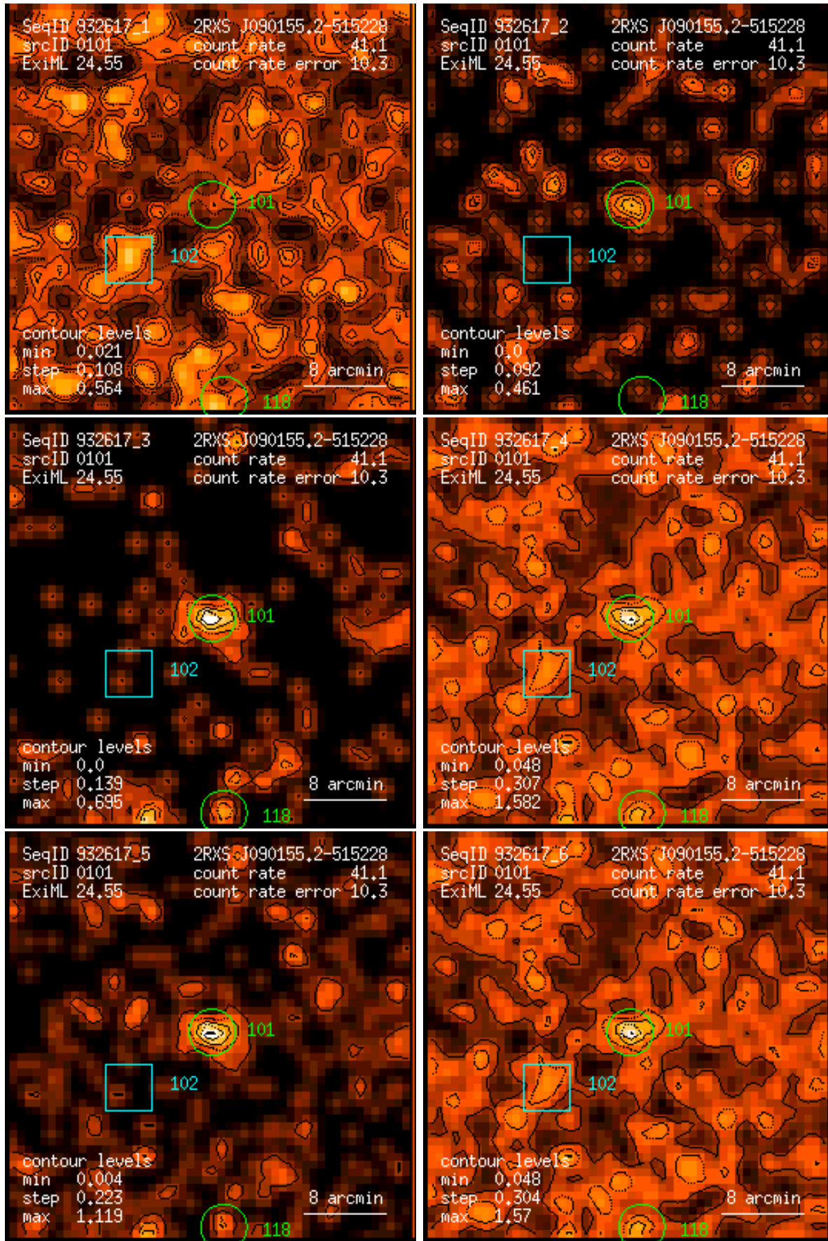
Figure 101: RASS 932617: detection 0101: band rate images, Gaussian filter: (1) PSPC channels 11 – 41, (2) 52 – 90, (3) 91 – 201, (4) 11 – 235, (5) 52 – 201, (6) 11 – 201. Broad band rates in counts/ks. Band rate contour levels in counts/ks/arcmin 2 .
