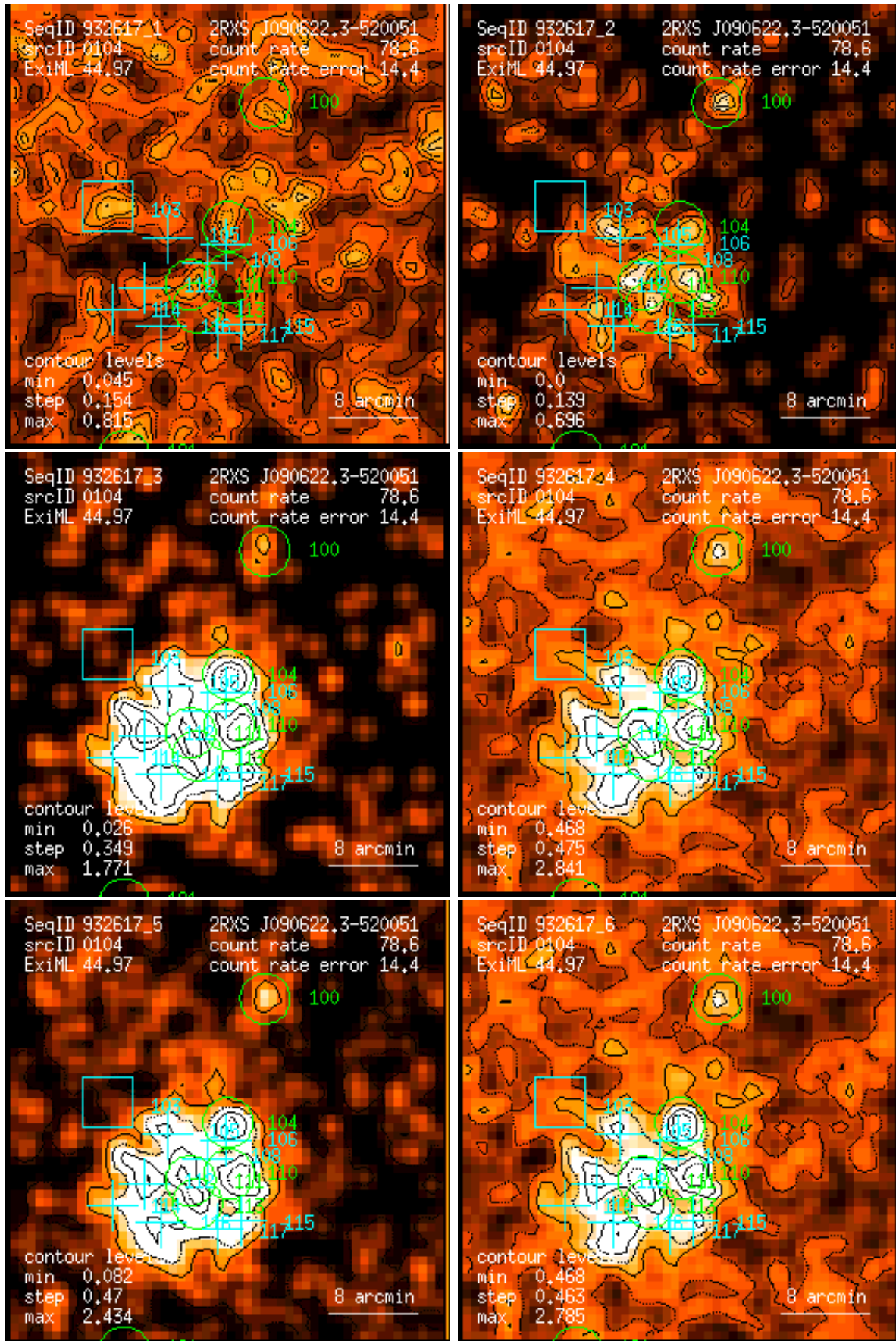
Figure 104: RASS 932617: detection 0104: band rate images, Gaussian filter: (1) PSPC channels 11 – 41, (2) 52 – 90, (3) 91 – 201, (4) 11 – 235, (5) 52 – 201, (6) 11 – 201. Broad band rates in counts/ks. Band rate contour levels in counts/ks/arcmin 2 .
