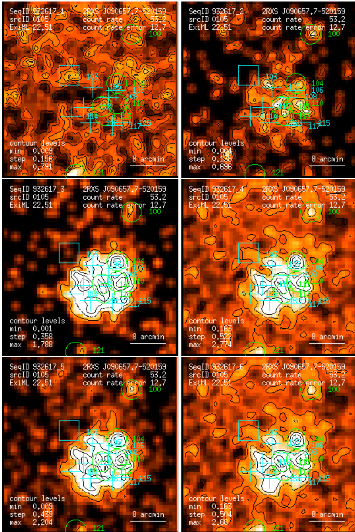
Figure 105: RASS 932617: detection 0105: band rate images, Gaussian filter: (1) PSPC channels 11 – 41, (2) 52 – 90, (3) 91 – 201, (4) 11 – 235, (5) 52 – 201, (6) 11 – 201. Broad band rates in counts/ks. Band rate contour levels in counts/ks/arcmin 2 .
