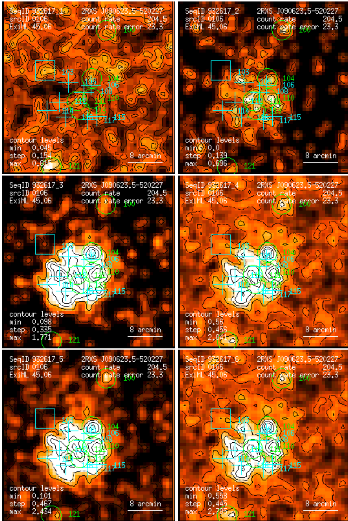
Figure 106: RASS 932617: detection 0106: band rate images, Gaussian filter: (1) PSPC channels 11 – 41, (2) 52 – 90, (3) 91 – 201, (4) 11 – 235, (5) 52 – 201, (6) 11 – 201. Broad band rates in counts/ks. Band rate contour levels in counts/ks/arcmin 2 .
