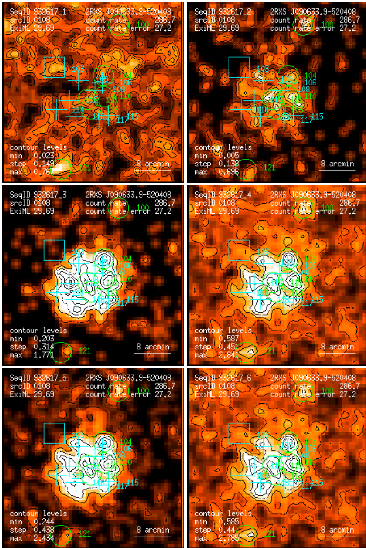
Figure 108: RASS 932617: detection 0108: band rate images, Gaussian filter: (1) PSPC channels 11 – 41, (2) 52 – 90, (3) 91 – 201, (4) 11 – 235, (5) 52 – 201, (6) 11 – 201. Broad band rates in counts/ks. Band rate contour levels in counts/ks/arcmin 2 .
