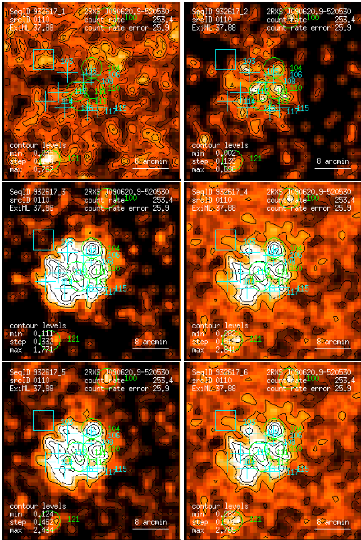
Figure 110: RASS 932617: detection 0110: band rate images, Gaussian filter: (1) PSPC channels 11 – 41, (2) 52 – 90, (3) 91 – 201, (4) 11 – 235, (5) 52 – 201, (6) 11 – 201. Broad band rates in counts/ks. Band rate contour levels in counts/ks/arcmin 2 .
