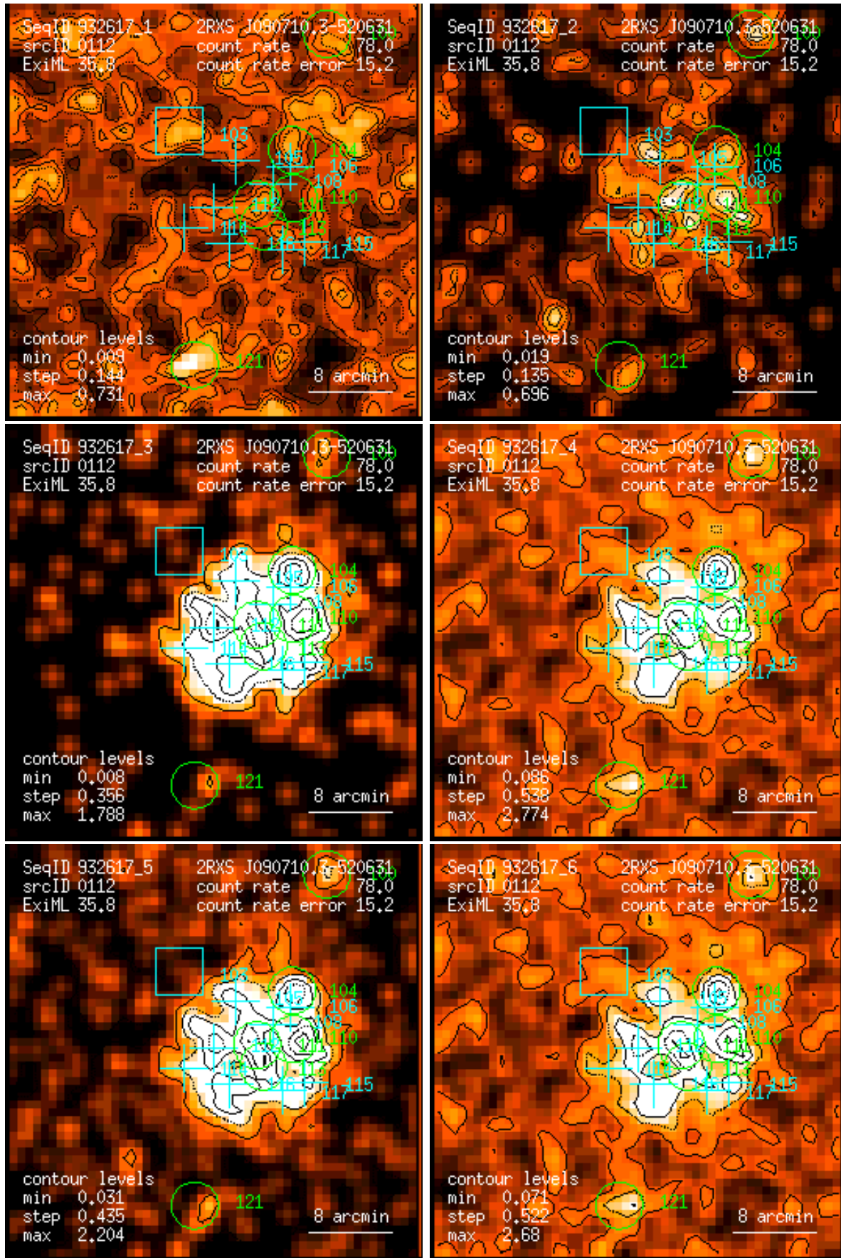
Figure 112: RASS 932617: detection 0112: band rate images, Gaussian filter: (1) PSPC channels 11 – 41, (2) 52 – 90, (3) 91 – 201, (4) 11 – 235, (5) 52 – 201, (6) 11 – 201. Broad band rates in counts/ks. Band rate contour levels in counts/ks/arcmin 2 .
