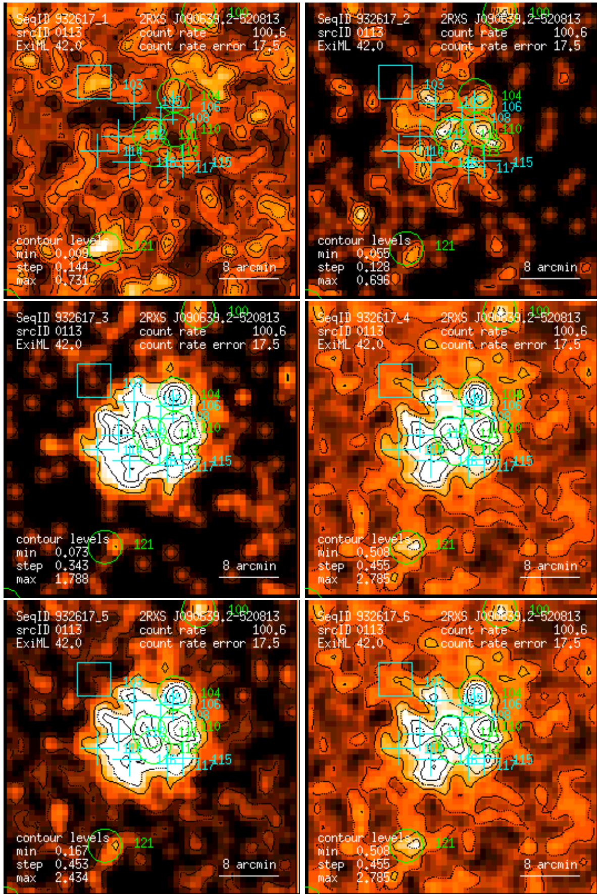
Figure 113: RASS 932617: detection 0113: band rate images, Gaussian filter: (1) PSPC channels 11 – 41, (2) 52 – 90, (3) 91 – 201, (4) 11 – 235, (5) 52 – 201, (6) 11 – 201. Broad band rates in counts/ks. Band rate contour levels in counts/ks/arcmin 2 .
