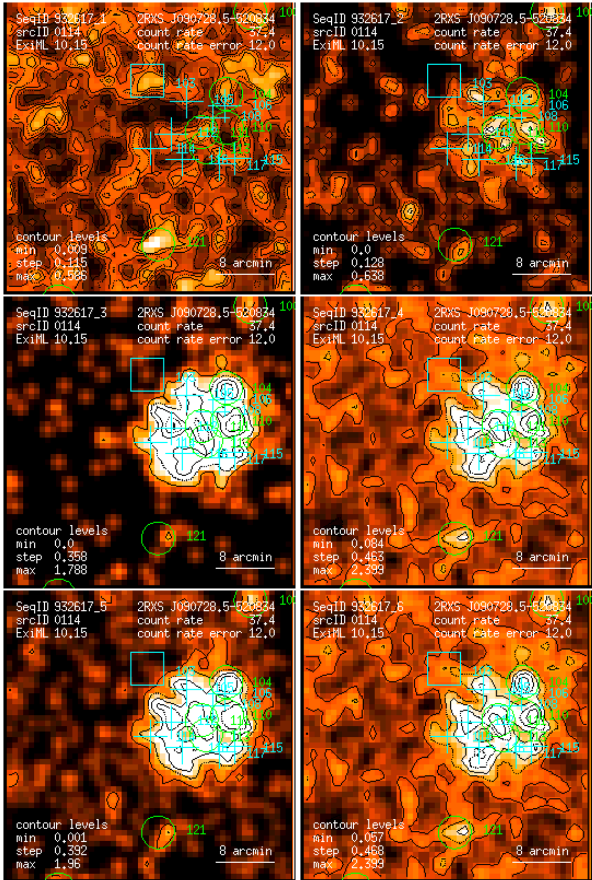
Figure 114: RASS 932617: detection 0114: band rate images, Gaussian filter: (1) PSPC channels 11 – 41, (2) 52 – 90, (3) 91 – 201, (4) 11 – 235, (5) 52 – 201, (6) 11 – 201. Broad band rates in counts/ks. Band rate contour levels in counts/ks/arcmin 2 .
