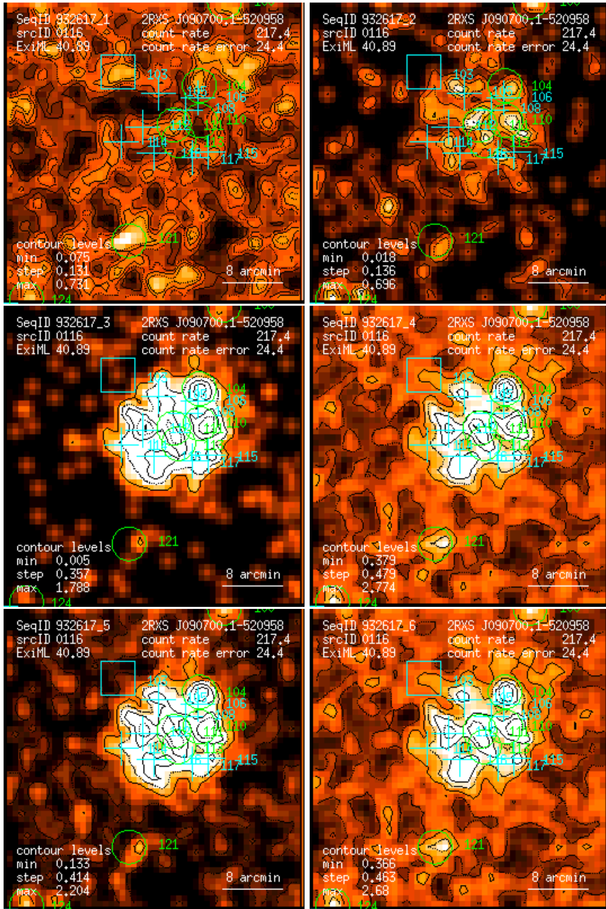
Figure 116: RASS 932617: detection 0116: band rate images, Gaussian filter: (1) PSPC channels 11 – 41, (2) 52 – 90, (3) 91 – 201, (4) 11 – 235, (5) 52 – 201, (6) 11 – 201. Broad band rates in counts/ks. Band rate contour levels in counts/ks/arcmin 2 .
