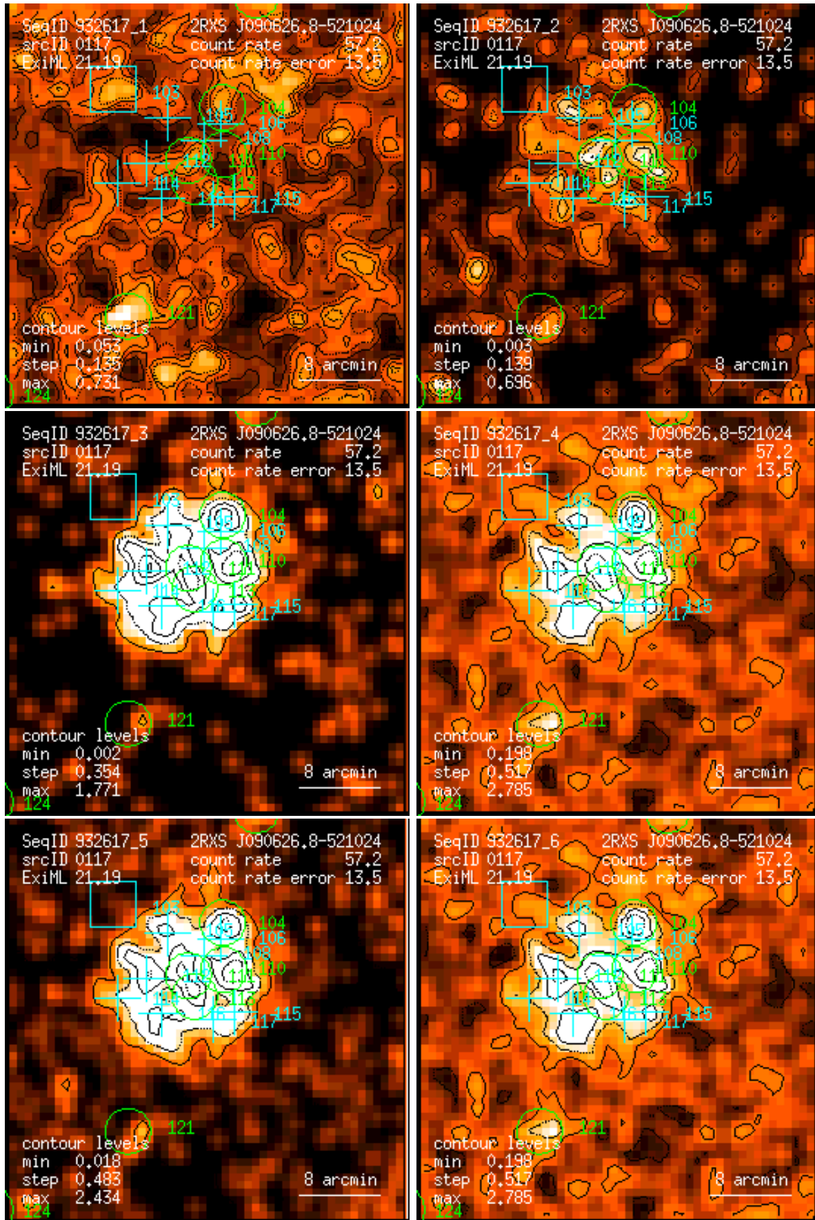
Figure 117: RASS 932617: detection 0117: band rate images, Gaussian filter: (1) PSPC channels 11 – 41, (2) 52 – 90, (3) 91 – 201, (4) 11 – 235, (5) 52 – 201, (6) 11 – 201. Broad band rates in counts/ks. Band rate contour levels in counts/ks/arcmin 2 .
