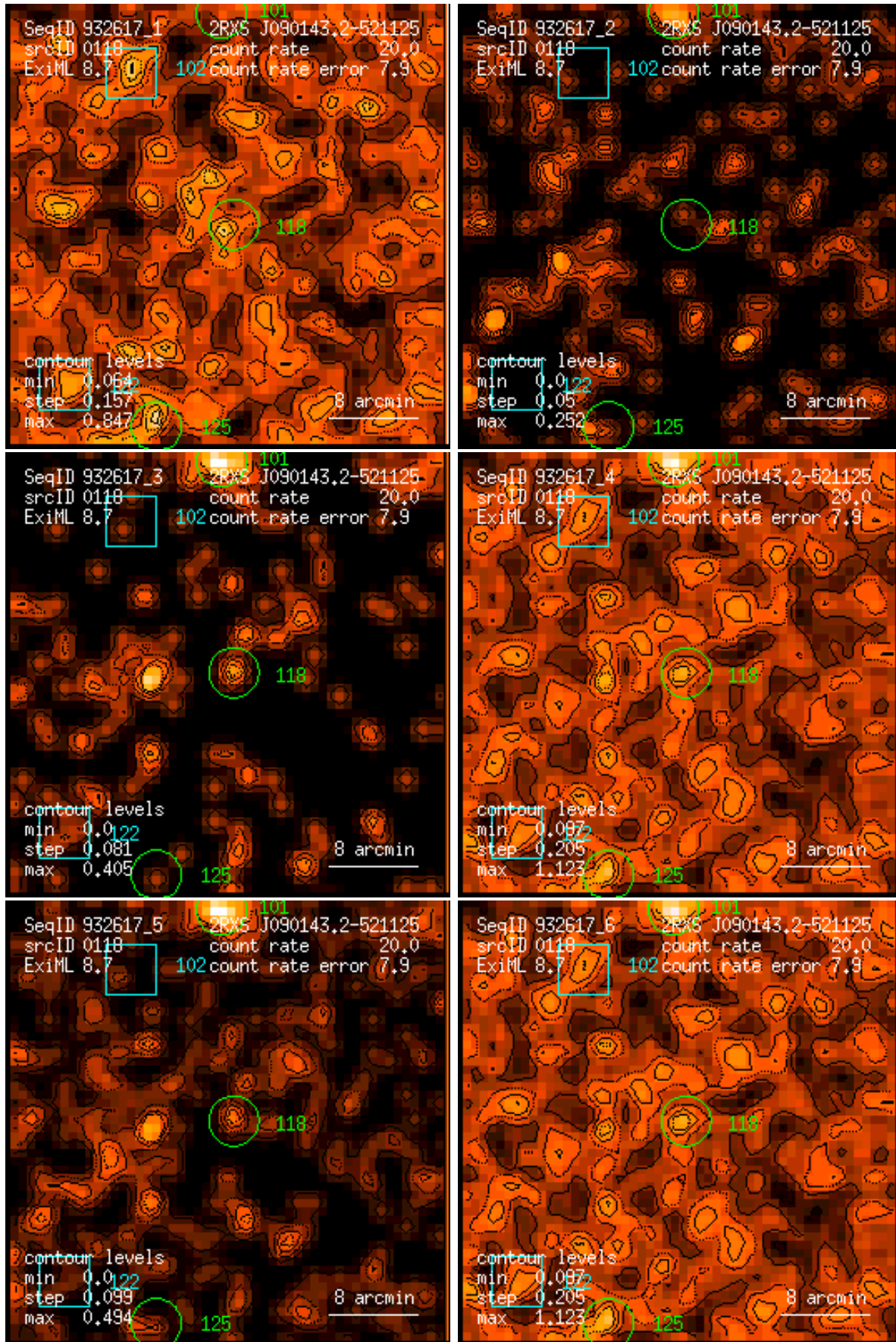
Figure 118: RASS 932617: detection 0118: band rate images, Gaussian filter: (1) PSPC channels 11 – 41, (2) 52 – 90, (3) 91 – 201, (4) 11 – 235, (5) 52 – 201, (6) 11 – 201. Broad band rates in counts/ks. Band rate contour levels in counts/ks/arcmin 2 .
