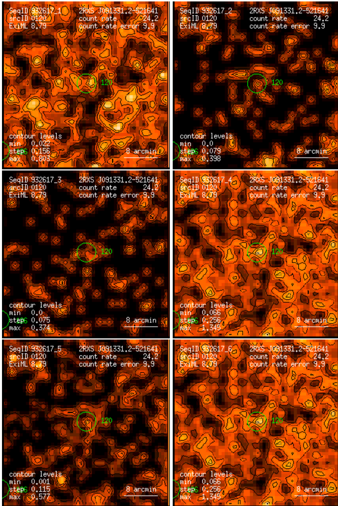
Figure 120: RASS 932617: detection 0120: band rate images, Gaussian filter: (1) PSPC channels 11 – 41, (2) 52 – 90, (3) 91 – 201, (4) 11 – 235, (5) 52 – 201, (6) 11 – 201. Broad band rates in counts/ks. Band rate contour levels in counts/ks/arcmin 2 .
