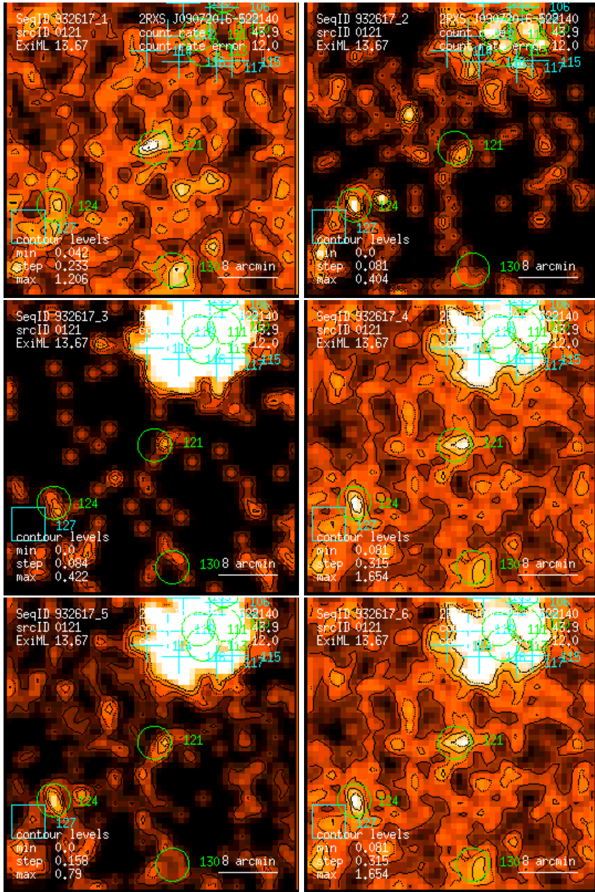
Figure 121: RASS 932617: detection 0121: band rate images, Gaussian filter: (1) PSPC channels 11 – 41, (2) 52 – 90, (3) 91 – 201, (4) 11 – 235, (5) 52 – 201, (6) 11 – 201. Broad band rates in counts/ks. Band rate contour levels in counts/ks/arcmin 2 .
