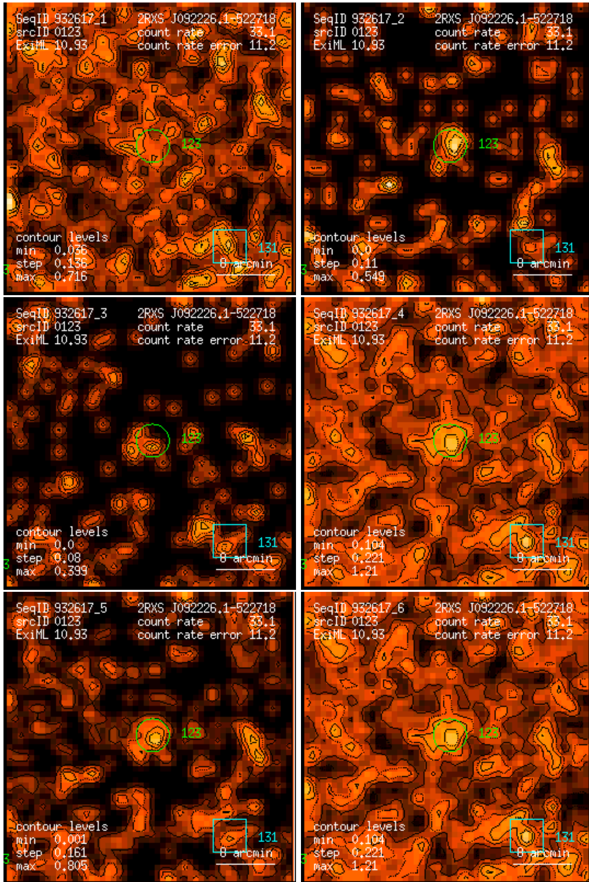
Figure 123: RASS 932617: detection 0123: band rate images, Gaussian filter: (1) PSPC channels 11 – 41, (2) 52 – 90, (3) 91 – 201, (4) 11 – 235, (5) 52 – 201, (6) 11 – 201. Broad band rates in counts/ks. Band rate contour levels in counts/ks/arcmin 2 .
