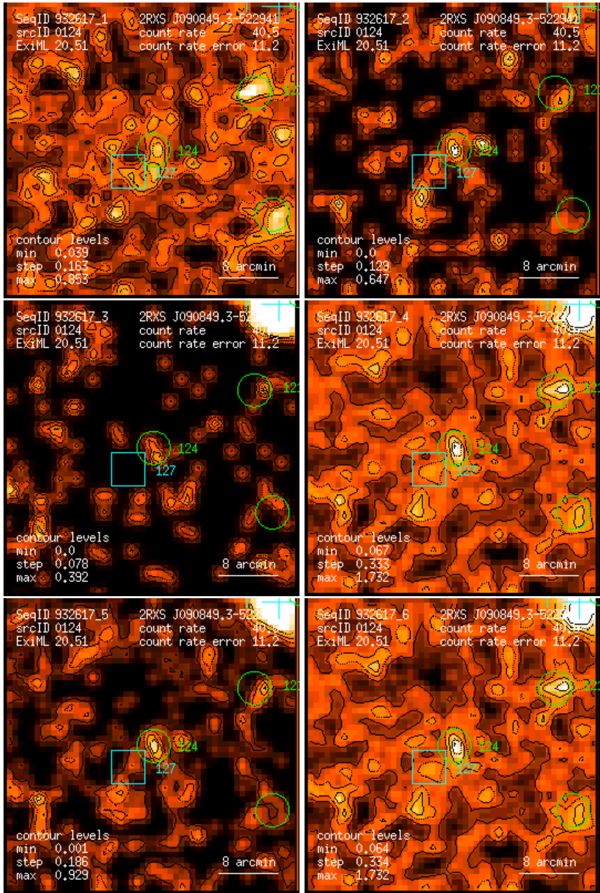
Figure 124: RASS 932617: detection 0124: band rate images, Gaussian filter: (1) PSPC channels 11 – 41, (2) 52 – 90, (3) 91 – 201, (4) 11 – 235, (5) 52 – 201, (6) 11 – 201. Broad band rates in counts/ks. Band rate contour levels in counts/ks/arcmin 2 .
