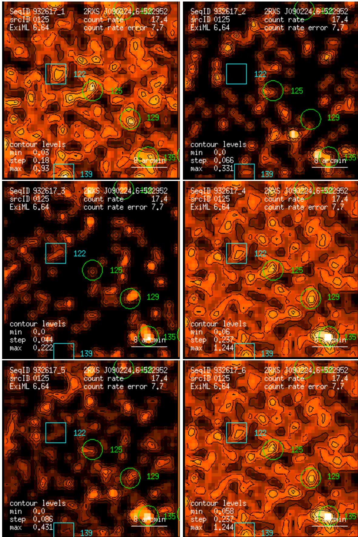
Figure 125: RASS 932617: detection 0125: band rate images, Gaussian filter: (1) PSPC channels 11 – 41, (2) 52 – 90, (3) 91 – 201, (4) 11 – 235, (5) 52 – 201, (6) 11 – 201. Broad band rates in counts/ks. Band rate contour levels in counts/ks/arcmin 2 .
