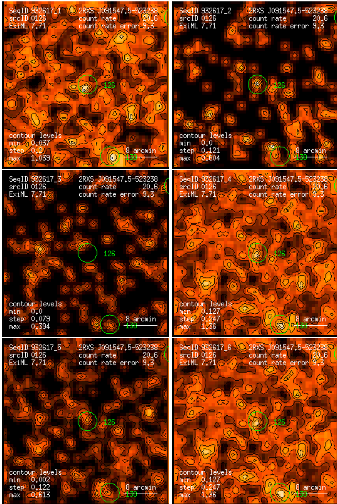
Figure 126: RASS 932617: detection 0126: band rate images, Gaussian filter: (1) PSPC channels 11 – 41, (2) 52 – 90, (3) 91 – 201, (4) 11 – 235, (5) 52 – 201, (6) 11 – 201. Broad band rates in counts/ks. Band rate contour levels in counts/ks/arcmin 2 .
