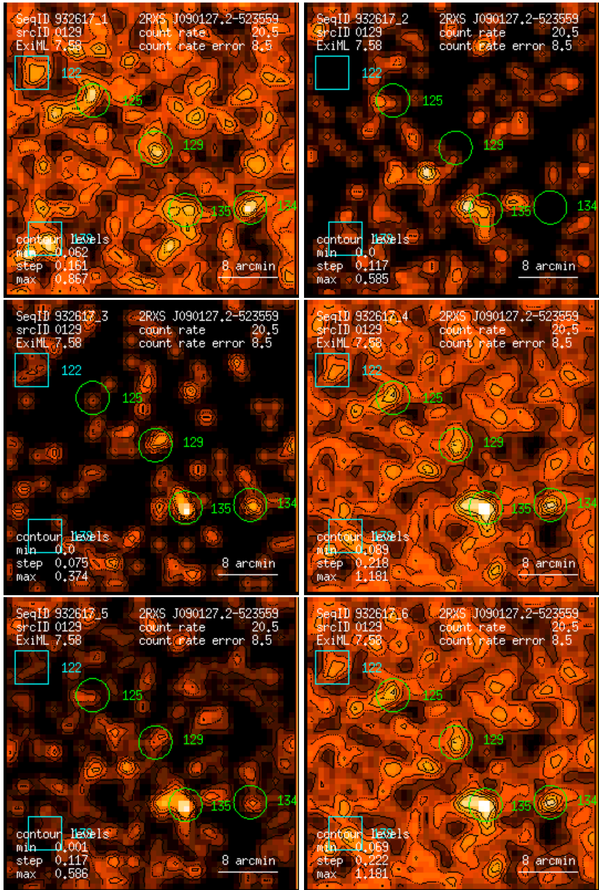
Figure 129: RASS 932617: detection 0129: band rate images, Gaussian filter: (1) PSPC channels 11 – 41, (2) 52 – 90, (3) 91 – 201, (4) 11 – 235, (5) 52 – 201, (6) 11 – 201. Broad band rates in counts/ks. Band rate contour levels in counts/ks/arcmin 2 .
