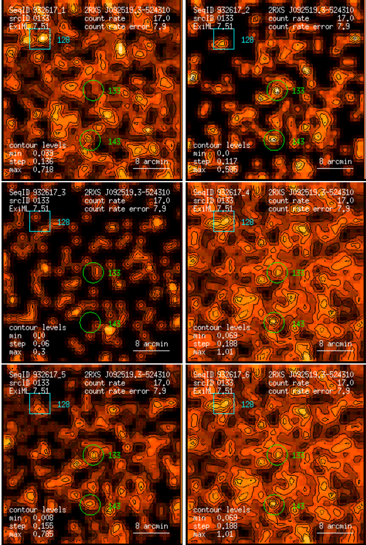
Figure 133: RASS 932617: detection 0133: band rate images, Gaussian filter: (1) PSPC channels 11 – 41, (2) 52 – 90, (3) 91 – 201, (4) 11 – 235, (5) 52 – 201, (6) 11 – 201. Broad band rates in counts/ks. Band rate contour levels in counts/ks/arcmin 2 .
