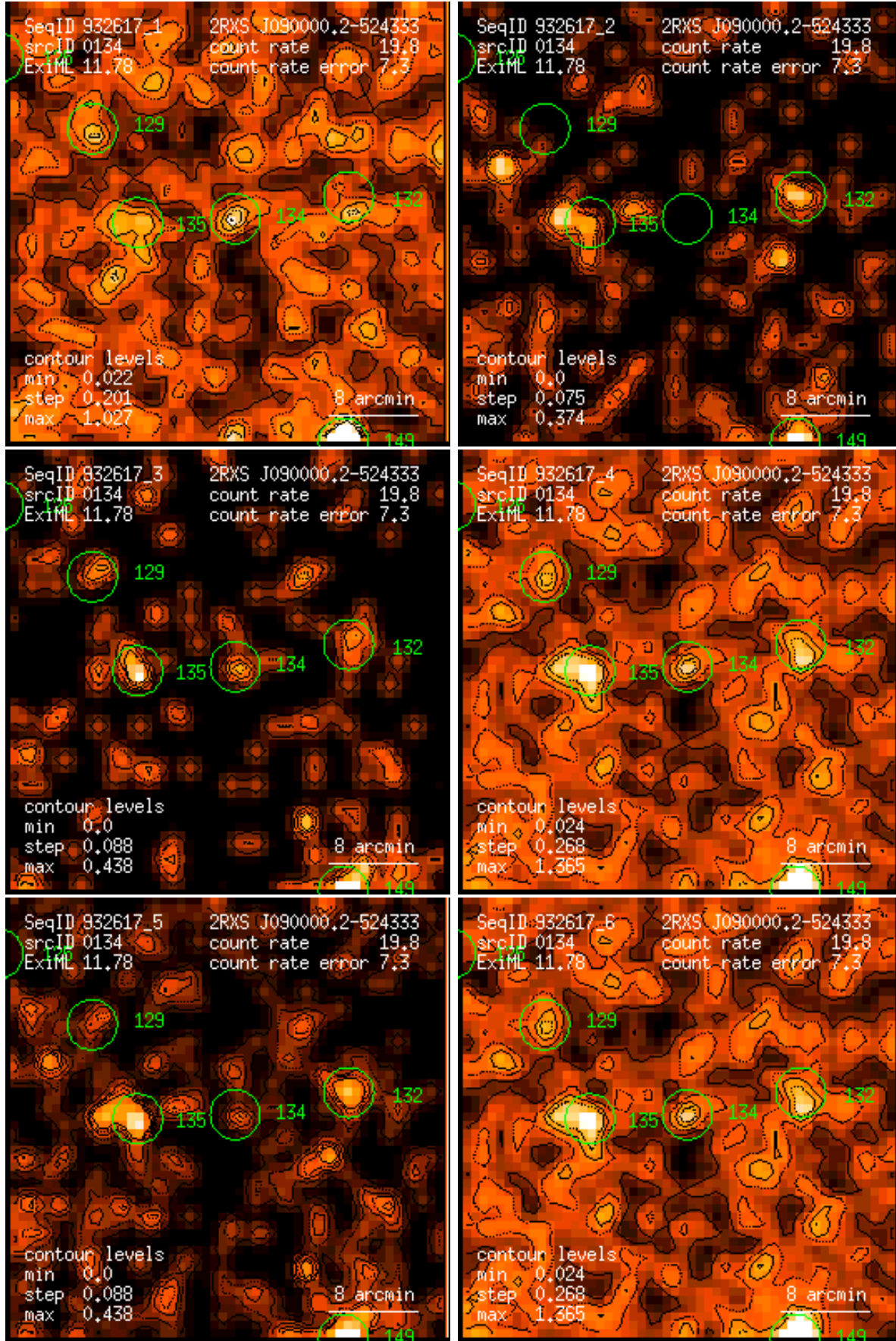
Figure 134: RASS 932617: detection 0134: band rate images, Gaussian filter: (1) PSPC channels 11 – 41, (2) 52 – 90, (3) 91 – 201, (4) 11 – 235, (5) 52 – 201, (6) 11 – 201. Broad band rates in counts/ks. Band rate contour levels in counts/ks/arcmin 2 .
