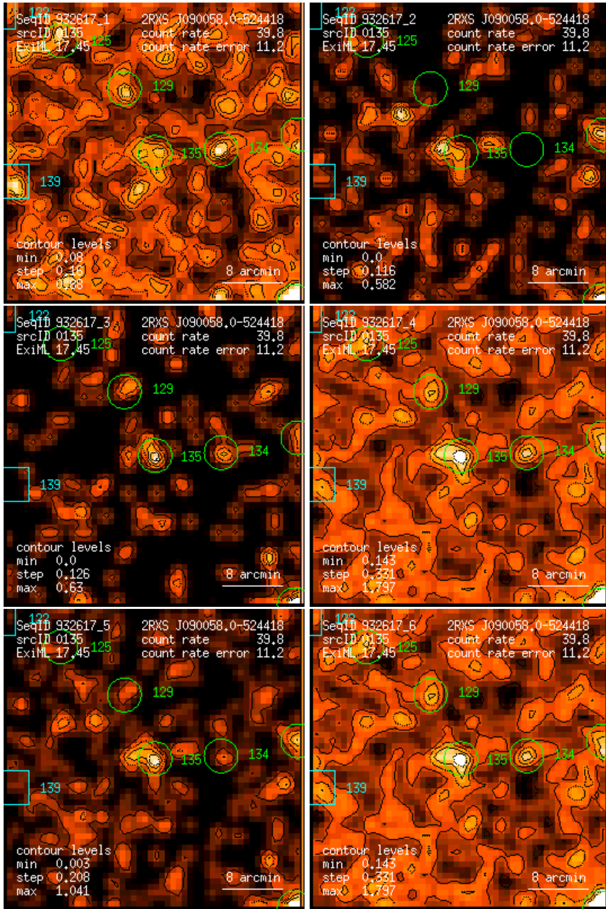
Figure 135: RASS 932617: detection 0135: band rate images, Gaussian filter: (1) PSPC channels 11 – 41, (2) 52 – 90, (3) 91 – 201, (4) 11 – 235, (5) 52 – 201, (6) 11 – 201. Broad band rates in counts/ks. Band rate contour levels in counts/ks/arcmin 2 .
