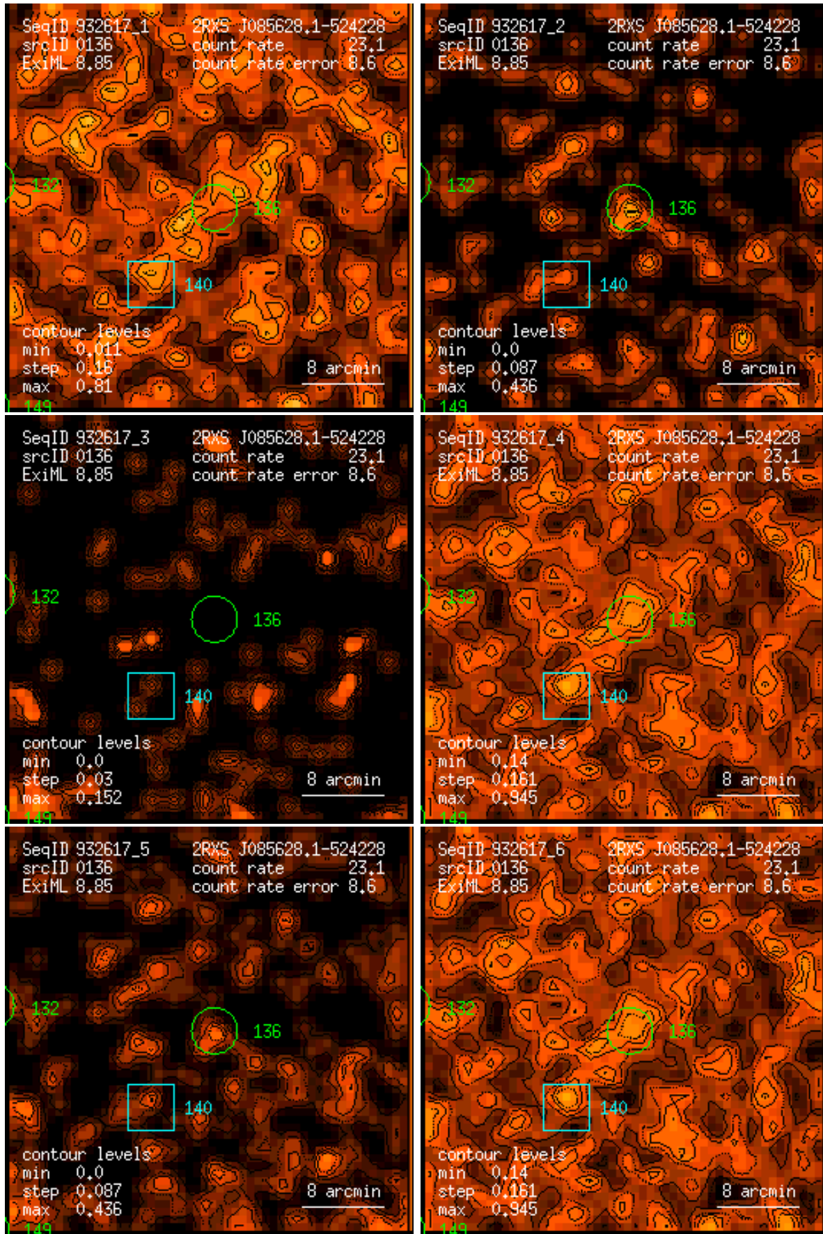
Figure 136: RASS 932617: detection 0136: band rate images, Gaussian filter: (1) PSPC channels 11 – 41, (2) 52 – 90, (3) 91 – 201, (4) 11 – 235, (5) 52 – 201, (6) 11 – 201. Broad band rates in counts/ks. Band rate contour levels in counts/ks/arcmin 2 .
