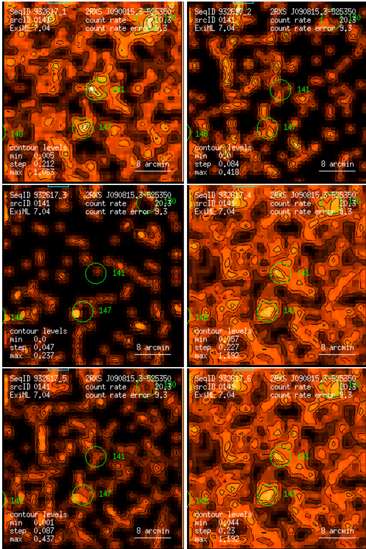
Figure 141: RASS 932617: detection 0141: band rate images, Gaussian filter: (1) PSPC channels 11 – 41, (2) 52 – 90, (3) 91 – 201, (4) 11 – 235, (5) 52 – 201, (6) 11 – 201. Broad band rates in counts/ks. Band rate contour levels in counts/ks/arcmin 2 .
