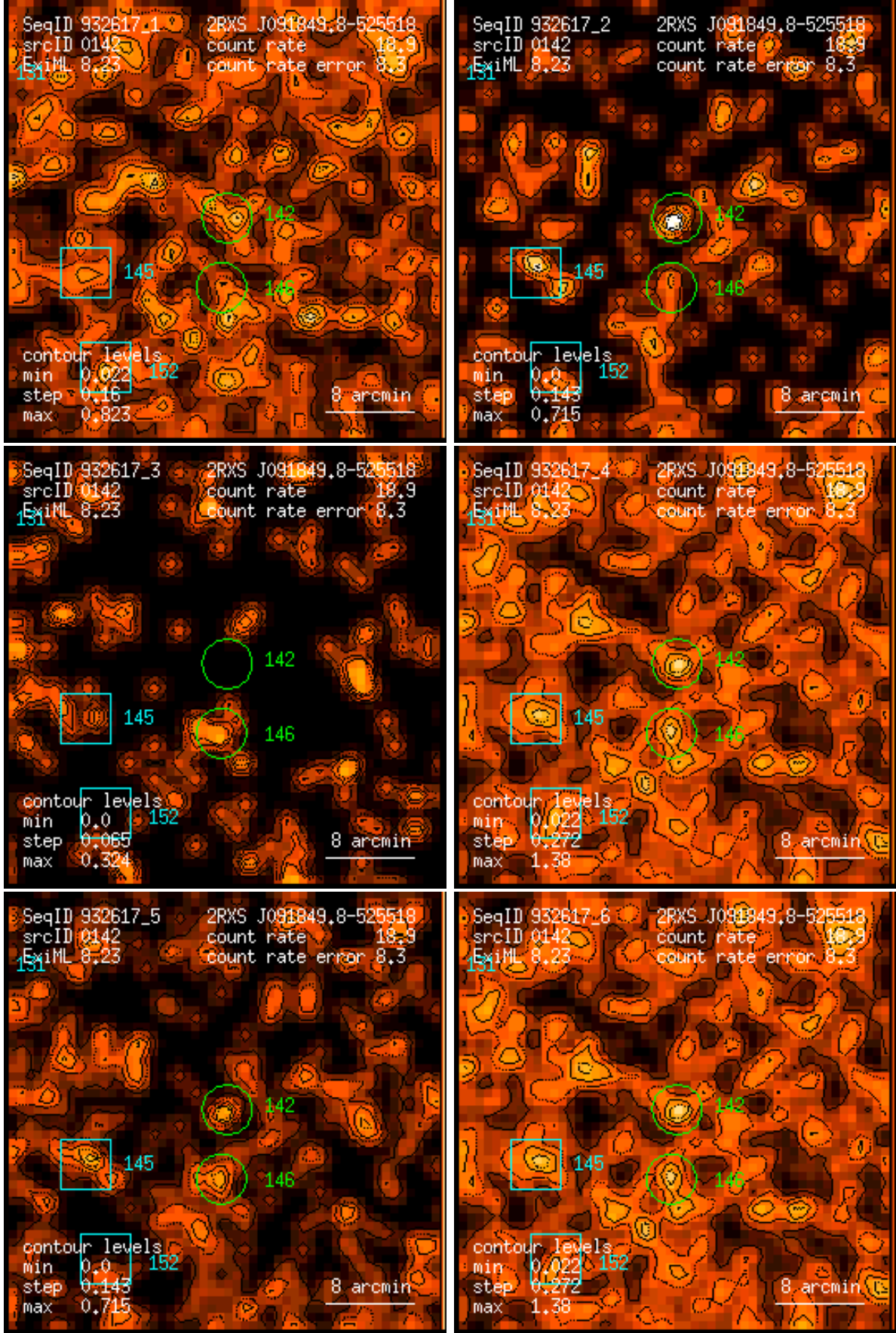
Figure 142: RASS 932617: detection 0142: band rate images, Gaussian filter: (1) PSPC channels 11 – 41, (2) 52 – 90, (3) 91 – 201, (4) 11 – 235, (5) 52 – 201, (6) 11 – 201. Broad band rates in counts/ks. Band rate contour levels in counts/ks/arcmin 2 .
